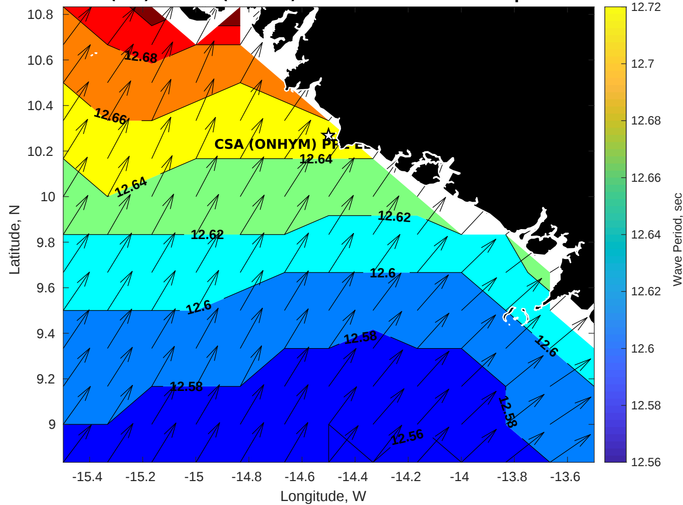
Wave Period (sec) for CSA (ONHYM) PPL EBS - Guinea at 12-Apr-2025 09:00:00
