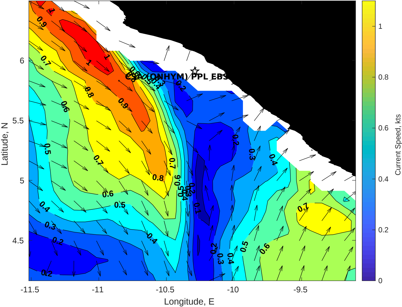
Surface Currents for CSA (ONHYM) PPL EBS - Liberia at 11-Apr-2025 00:00:00
