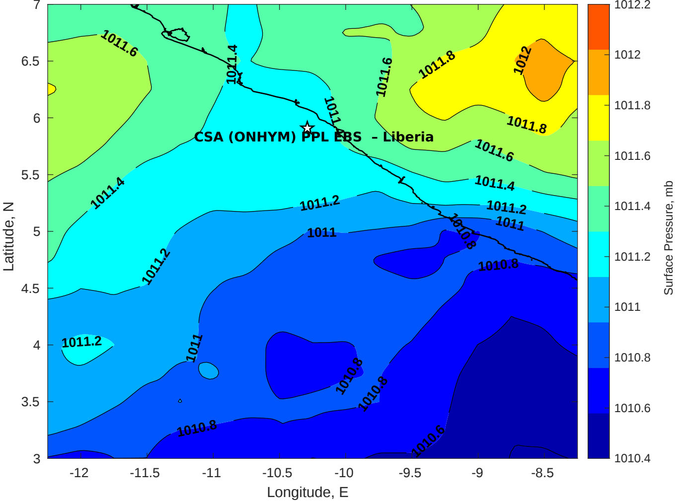
Surface Pressure (mb) for CSA (ONHYM) PPL EBS - Liberia at 12-Apr-2025 00:00:00
