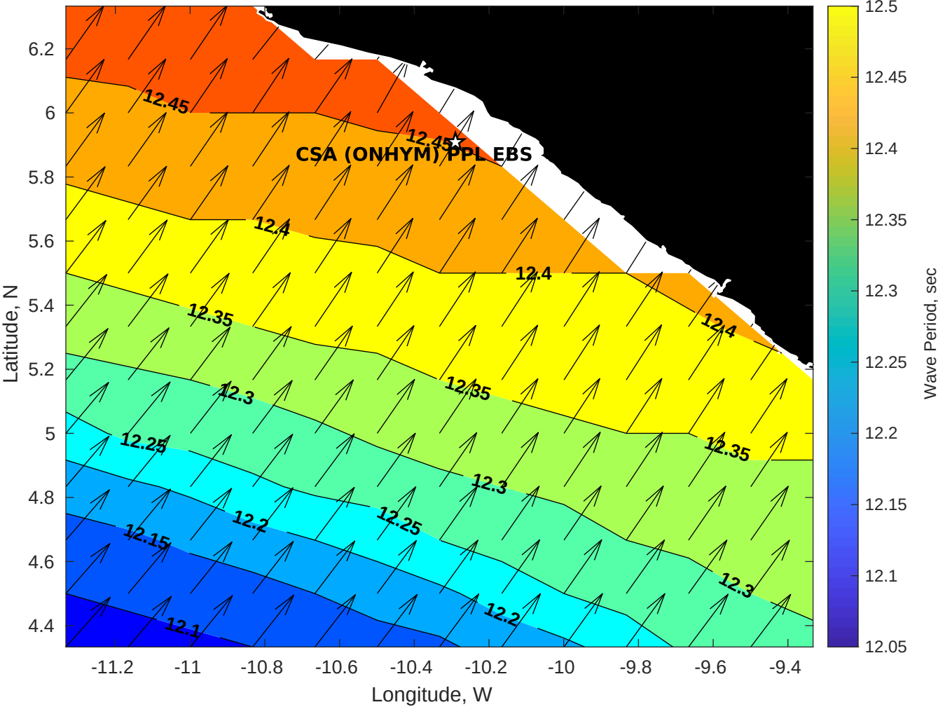
Wave Period (sec) for CSA (ONHYM) PPL EBS - Liberia at 12-Apr-2025 09:00:00
