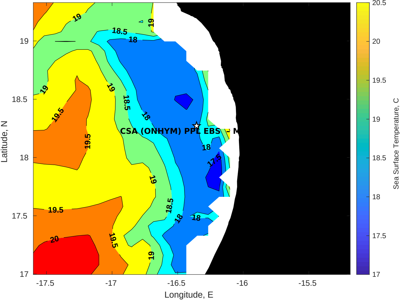
SST for CSA (ONHYM) PPL EBS - Mauritania at 11-Apr-2025 00:00:00
