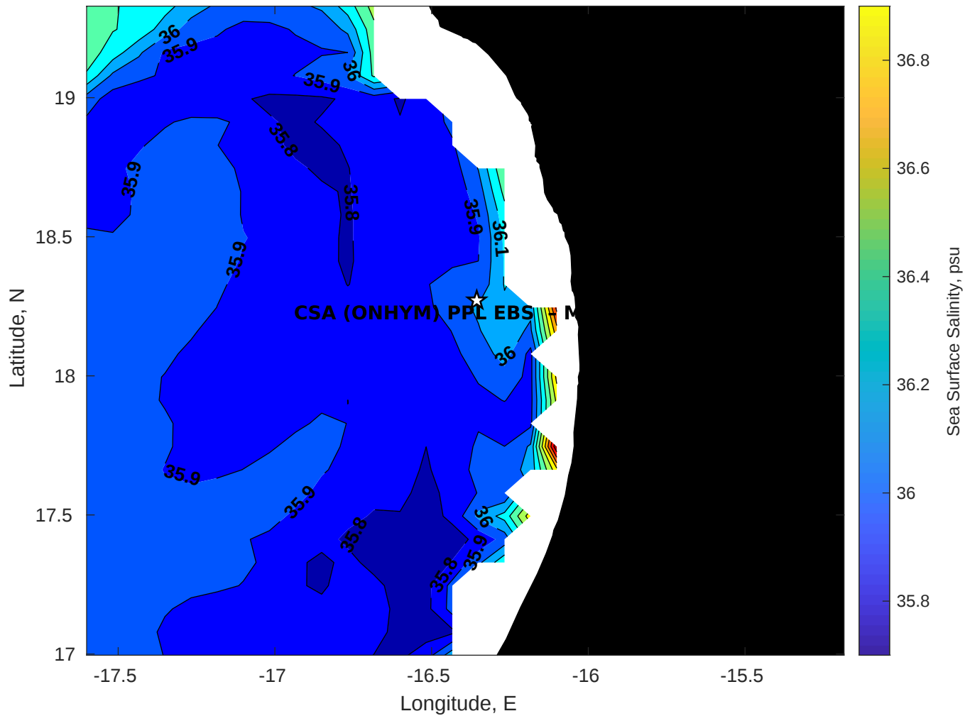
Surface Salinity for CSA (ONHYM) PPL EBS - Mauritania at 11-Apr-2025 00:00:00
