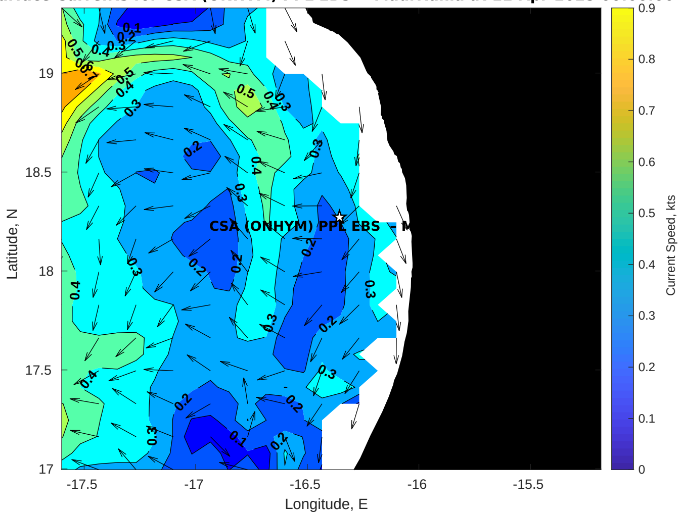
Surface Currents for CSA (ONHYM) PPL EBS - Mauritania at 11-Apr-2025 00:00:00
