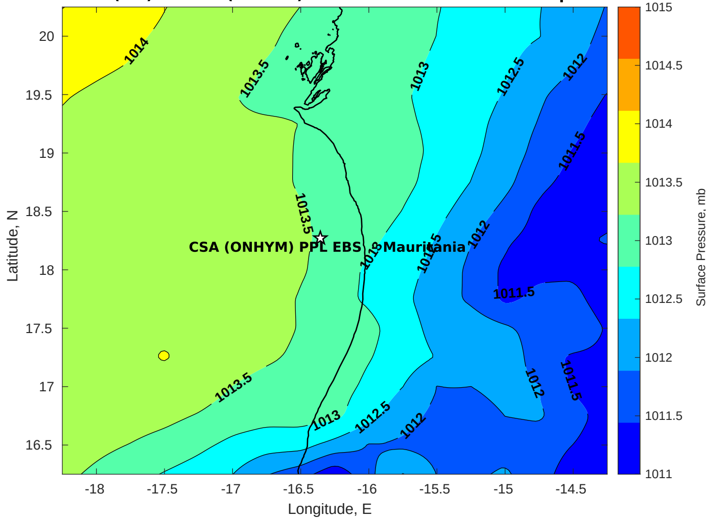
Surface Pressure (mb) for CSA (ONHYM) PPL EBS - Mauritania at 12-Apr-2025 00:00:00
