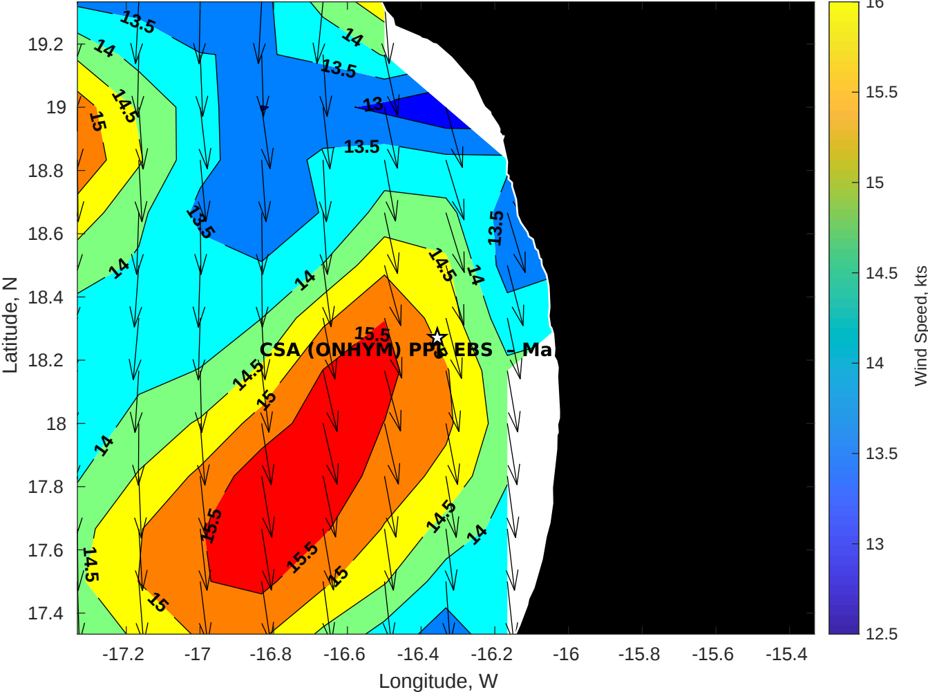
Winds (kts) for CSA (ONHYM) PPL EBS - Mauritania at 12-Apr-2025 09:00:00
