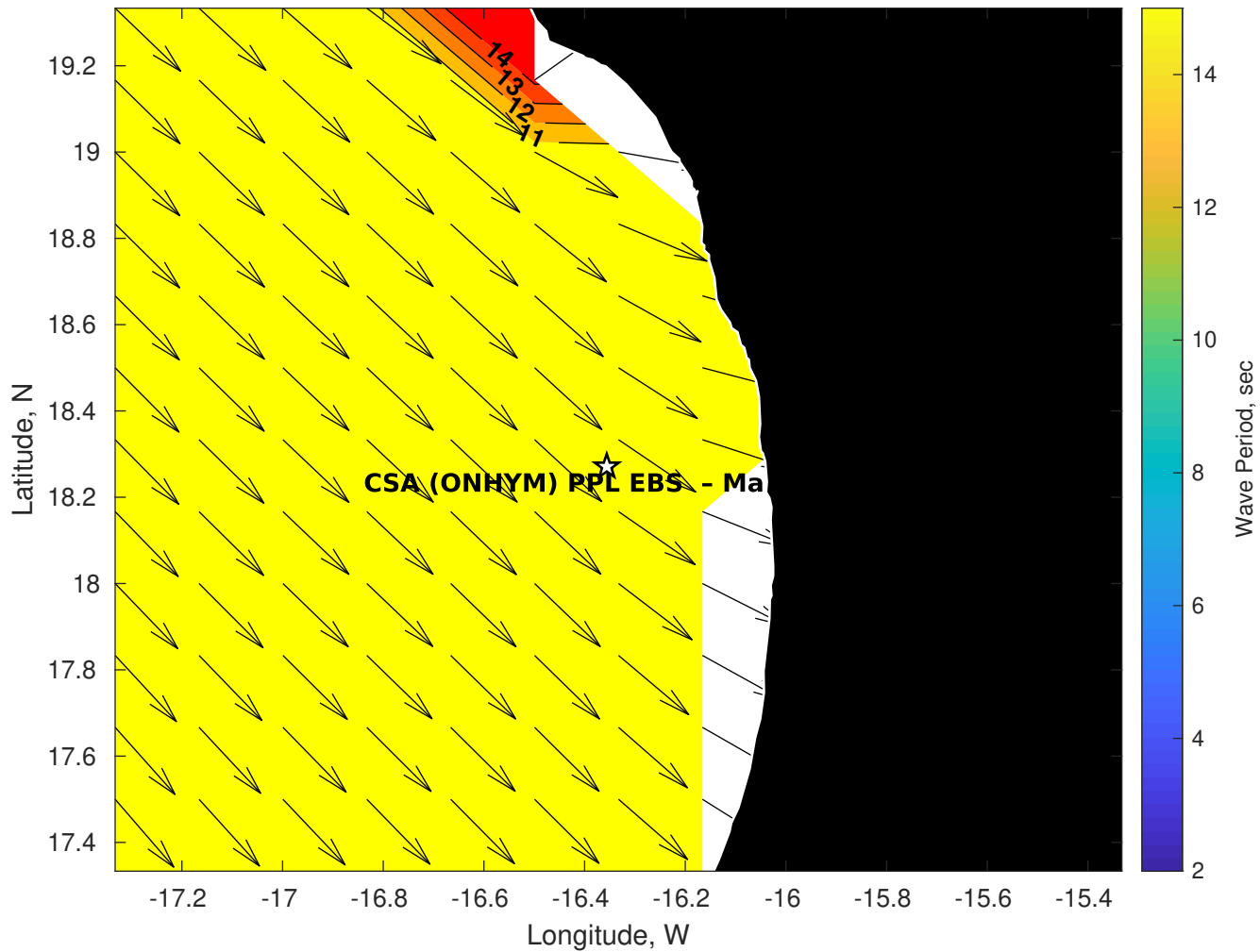
Wave Period (sec) for CSA (ONHYM) PPL EBS - Mauritania at 12-Apr-2025 09:00:00
