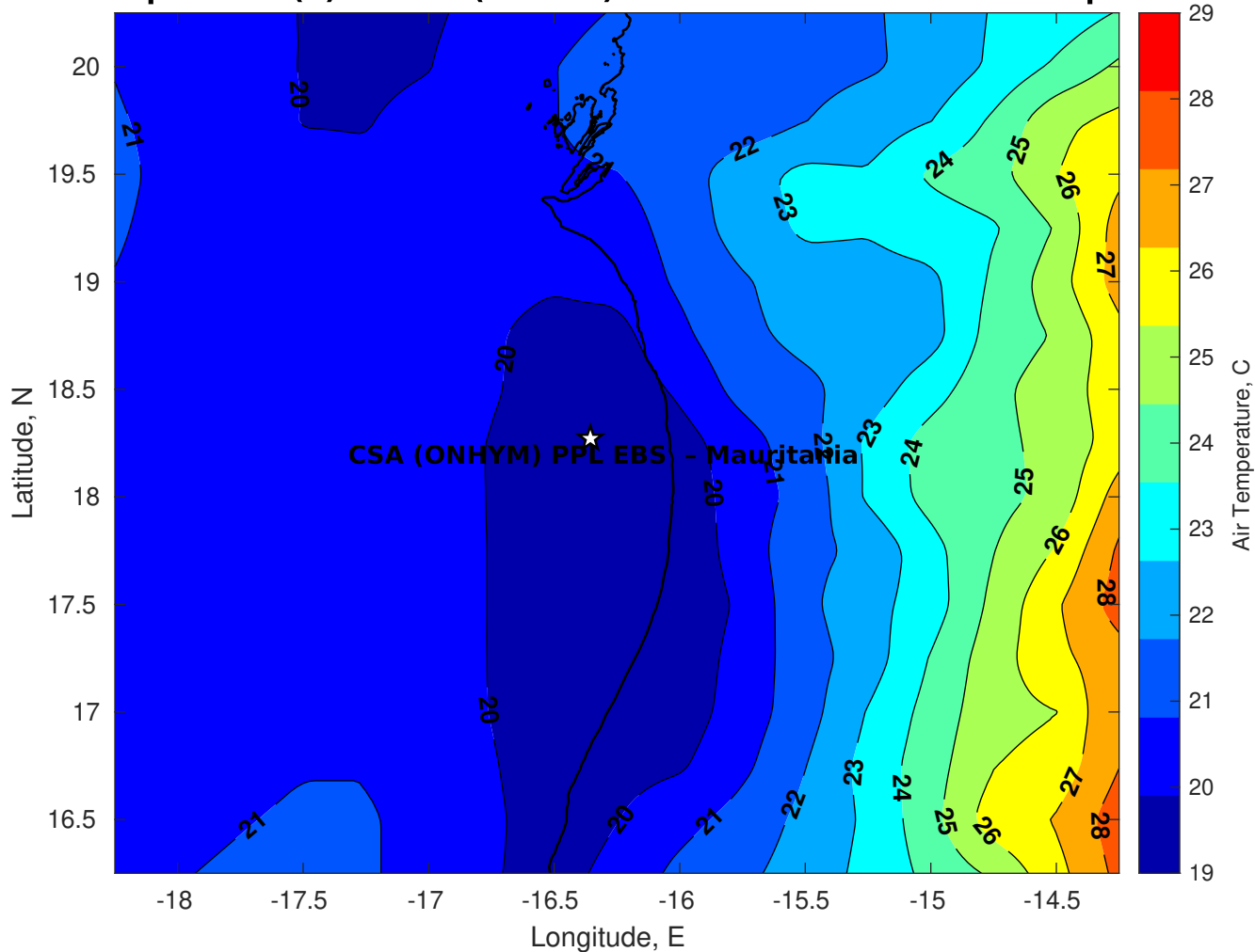
Air Temperature (C) for CSA (ONHYM) PPL EBS - Mauritania at 12-Apr-2025
