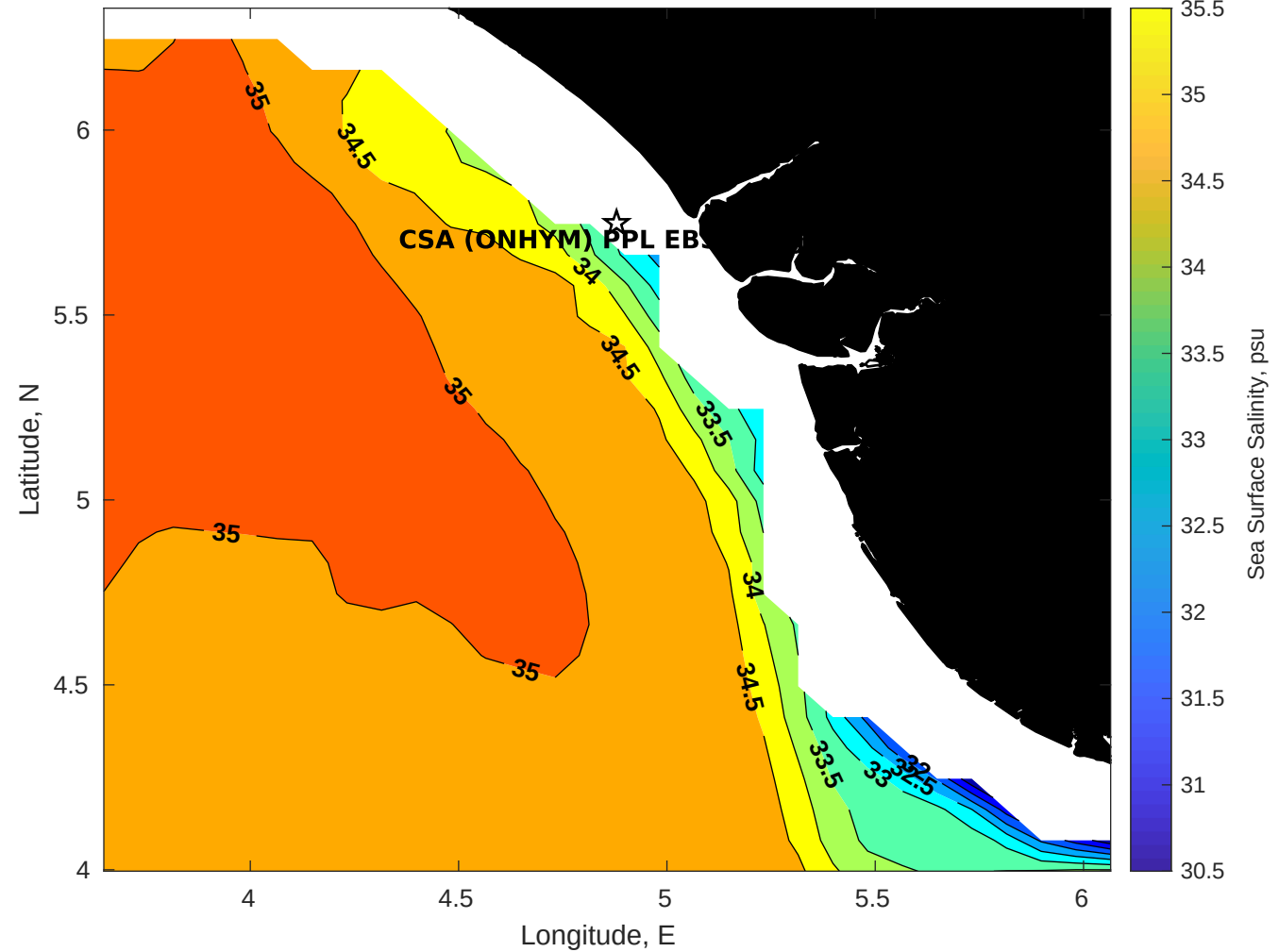
Surface Salinity for CSA (ONHYM) PPL EBS - Nigeria at 11-Apr-2025 00:00:00
