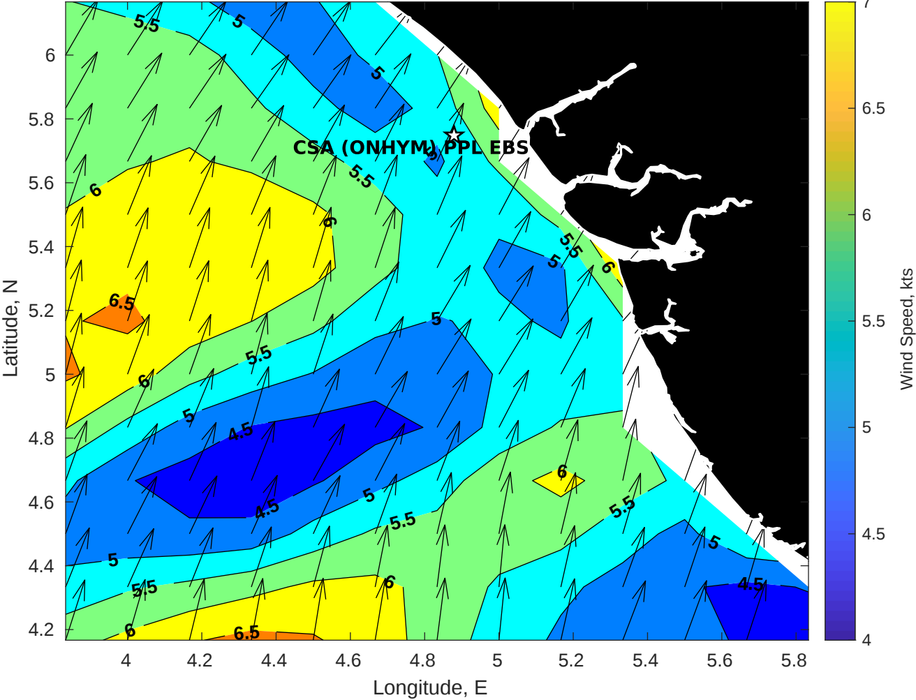
Winds (kts) for CSA (ONHYM) PPL EBS - Nigeria at 12-Apr-2025 09:00:00
