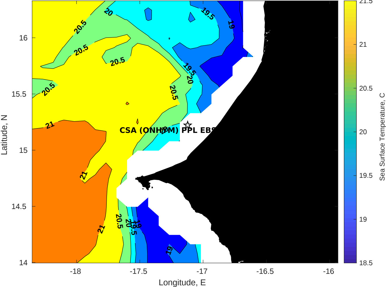
SST for CSA (ONHYM) PPL EBS - Senegal at 11-Apr-2025 00:00:00
