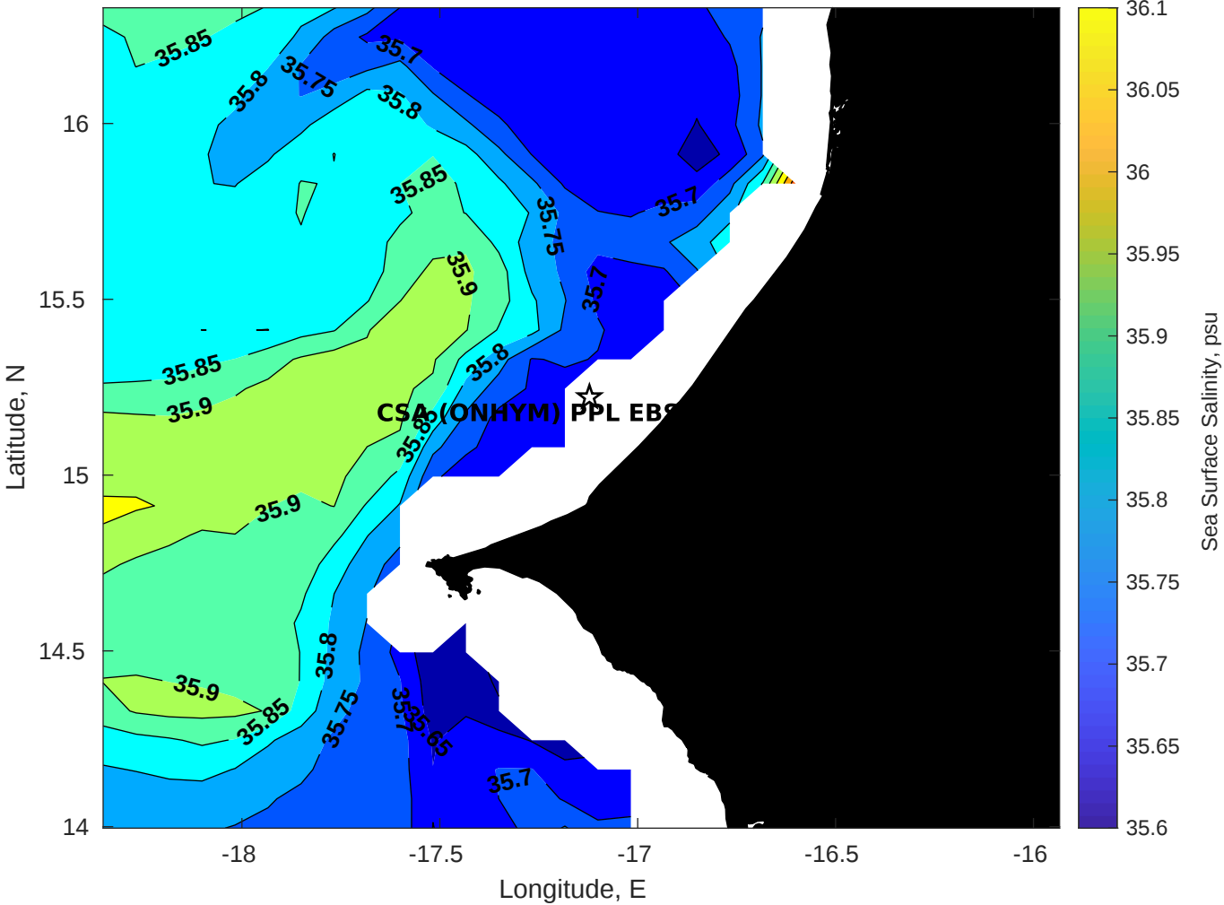
Surface Salinity for CSA (ONHYM) PPL EBS - Senegal at 11-Apr-2025 00:00:00
