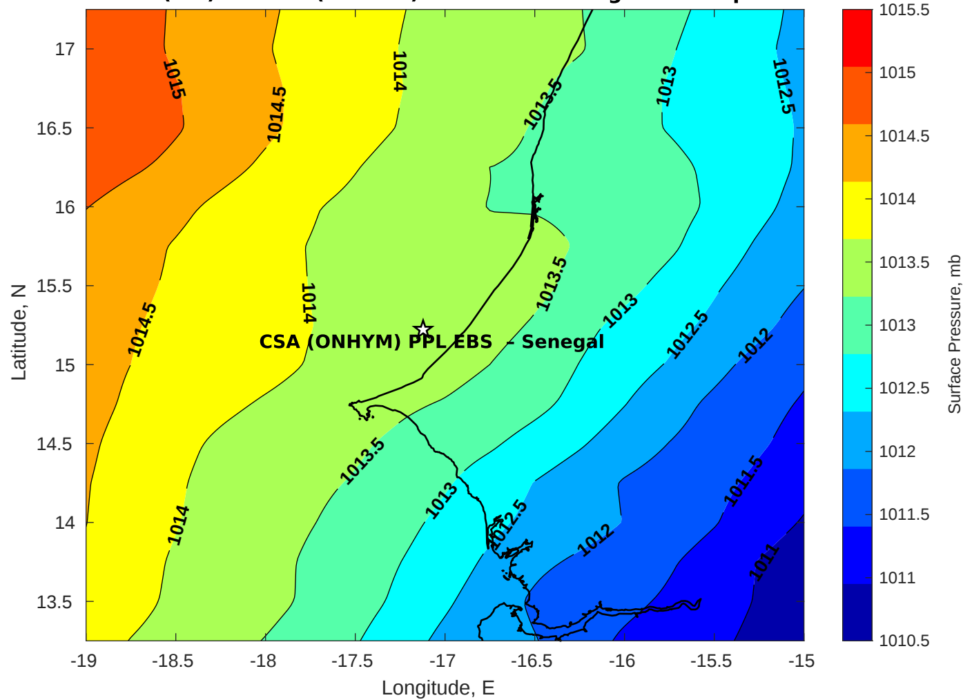
Surface Pressure (mb) for CSA (ONHYM) PPL EBS - Senegal at 14-Apr-2025 00:00:00
