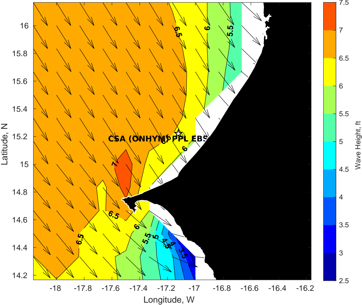
Wave Height (ft) for CSA (ONHYM) PPL EBS - Senegal at 12-Apr-2025 09:00:00
