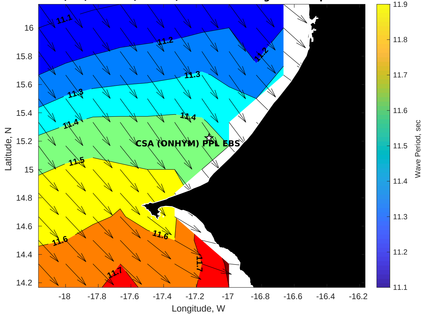
Wave Period (sec) for CSA (ONHYM) PPL EBS - Senegal at 12-Apr-2025 09:00:00
