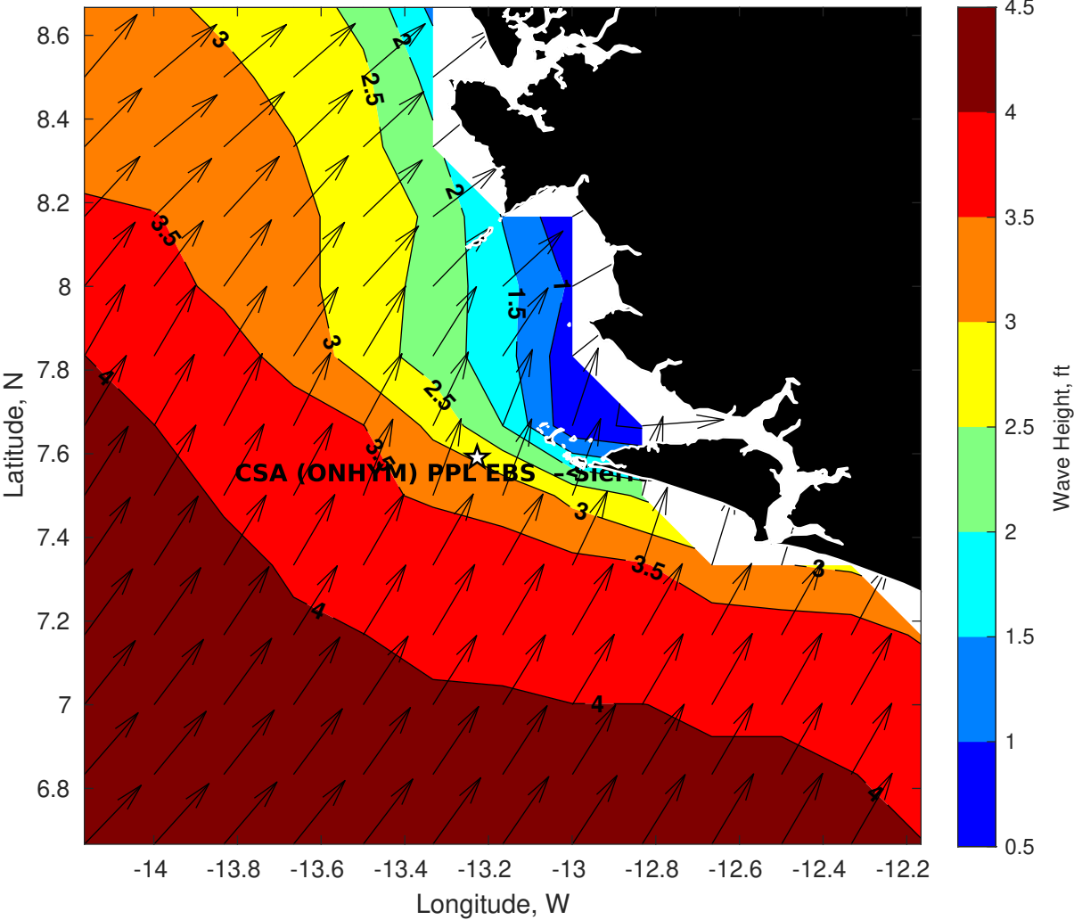
Wave Height (ft) for CSA (ONHYM) PPL EBS - Sierra Leone at 12-Apr-2025 09:00:00
