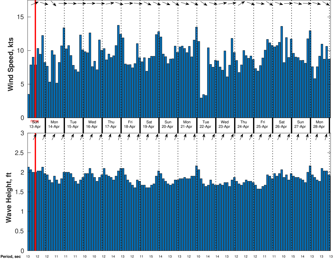
Wind & Wave Forecast for CSA (ONHYM) PPL EBS - Sierra Leone from 12-Apr-2025 01:00:00 to 28-Apr-2025 01:00:00
