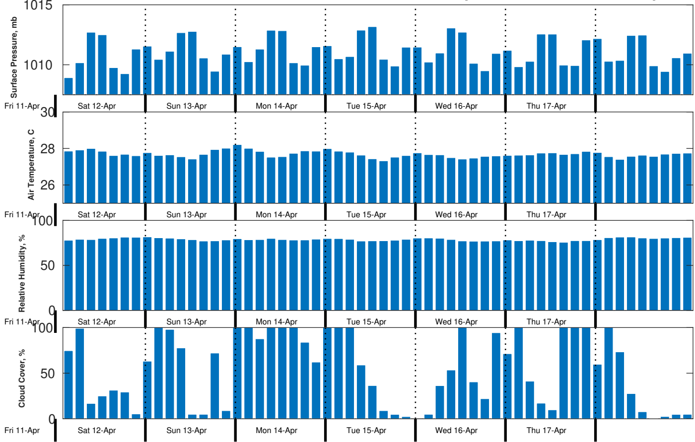
Met Forecast for CSA (ONHYM) PPL EBS - Sierra Leone from 12-Apr-2025 00:00:00 to 19-Apr-2025 00:00:00
