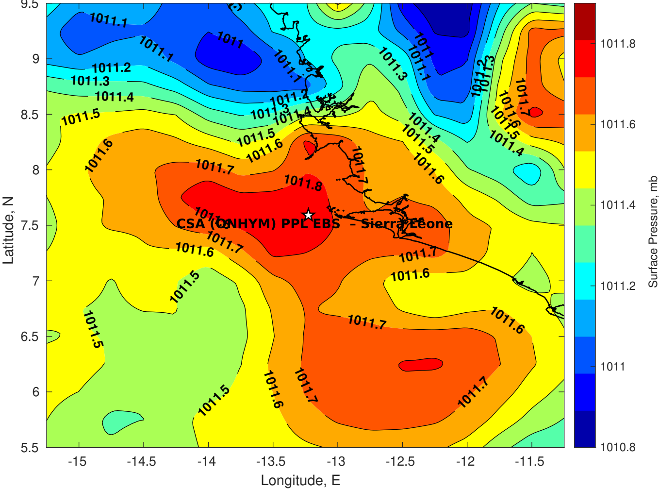
Surface Pressure (mb) for CSA (ONHYM) PPL EBS - Sierra Leone at 12-Apr-2025 00:00:00
