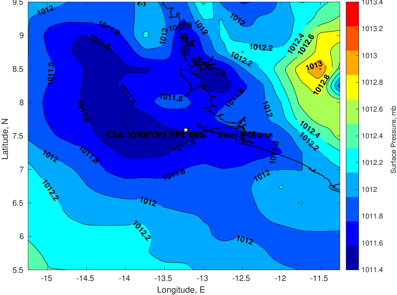
Surface Pressure (mb) for CSA (ONHYM) PPL EBS - Sierra Leone at 13-Apr-2025 00:00:00
