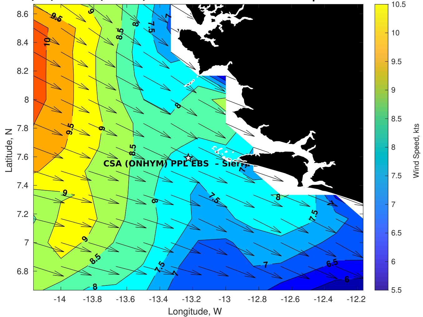
Winds (kts) for CSA (ONHYM) PPL EBS - Sierra Leone at 12-Apr-2025 09:00:00
