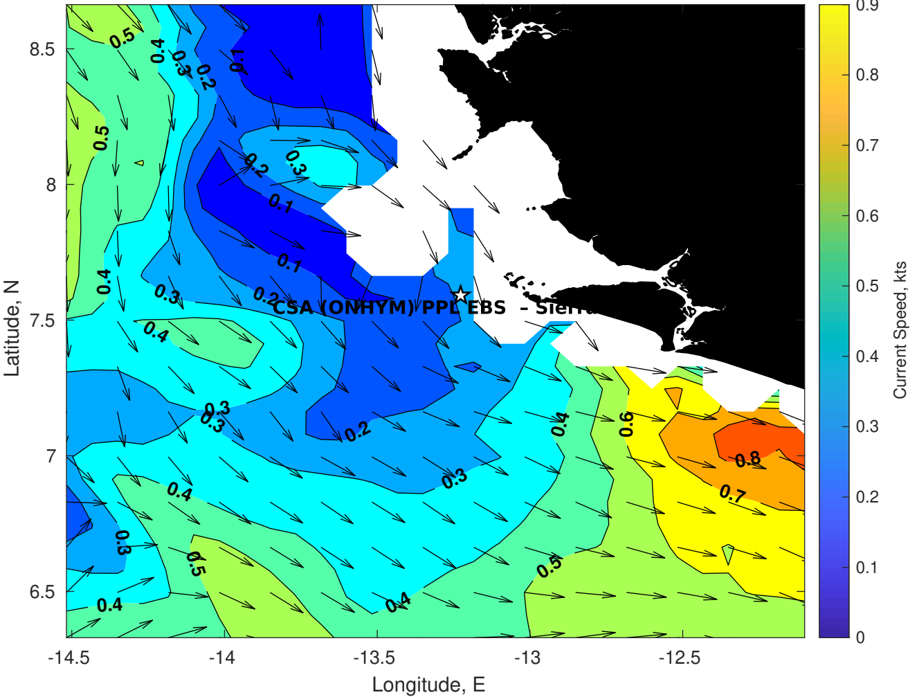
Surface Currents for CSA (ONHYM) PPL EBS - Sierra Leone at 11-Apr-2025 00:00:00
