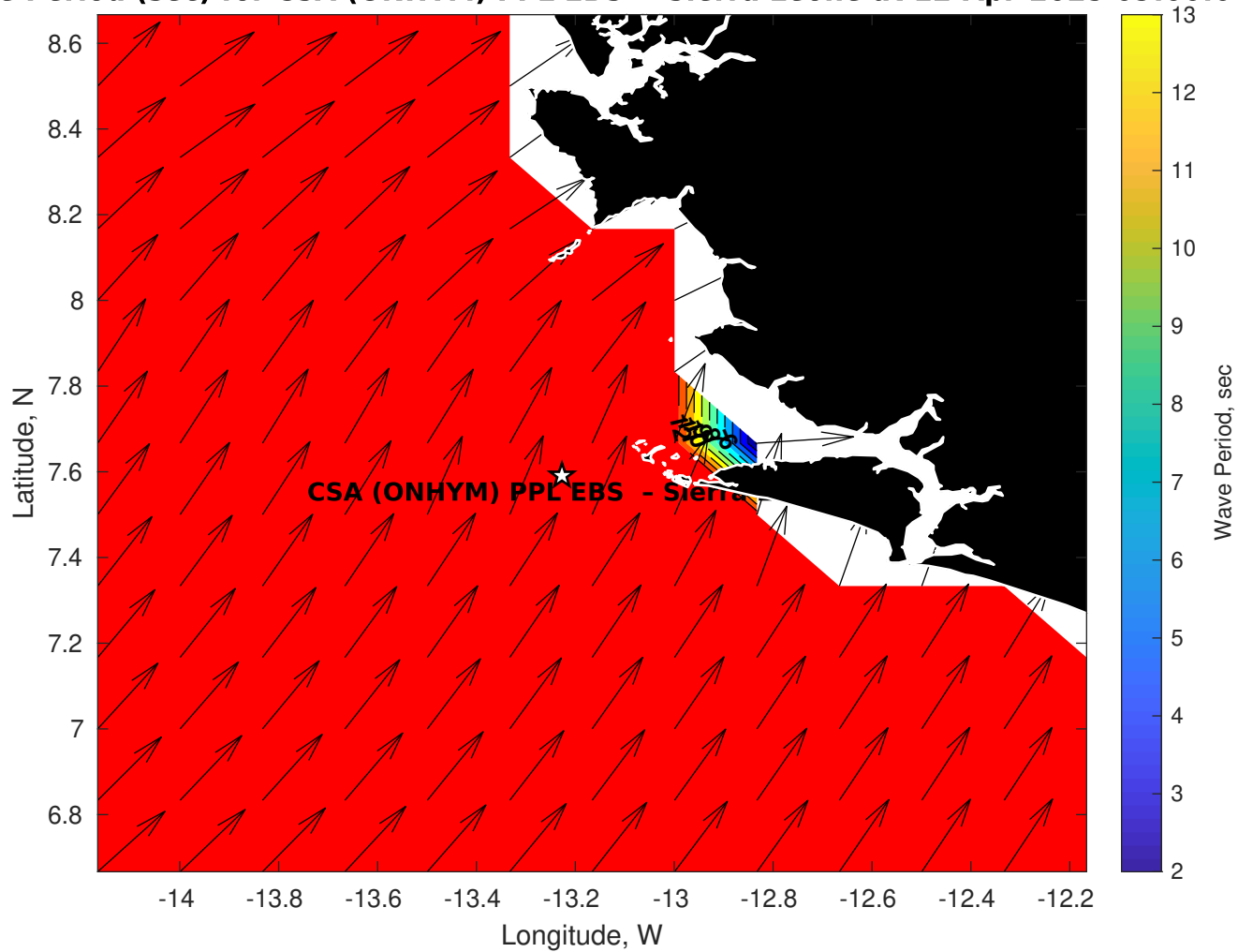
Wave Period (sec) for CSA (ONHYM) PPL EBS - Sierra Leone at 12-Apr-2025 09:00:00
