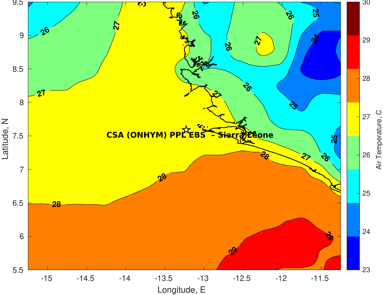
Air Temperature (C) for CSA (ONHYM) PPL EBS - Sierra Leone at 12-Apr-2025
