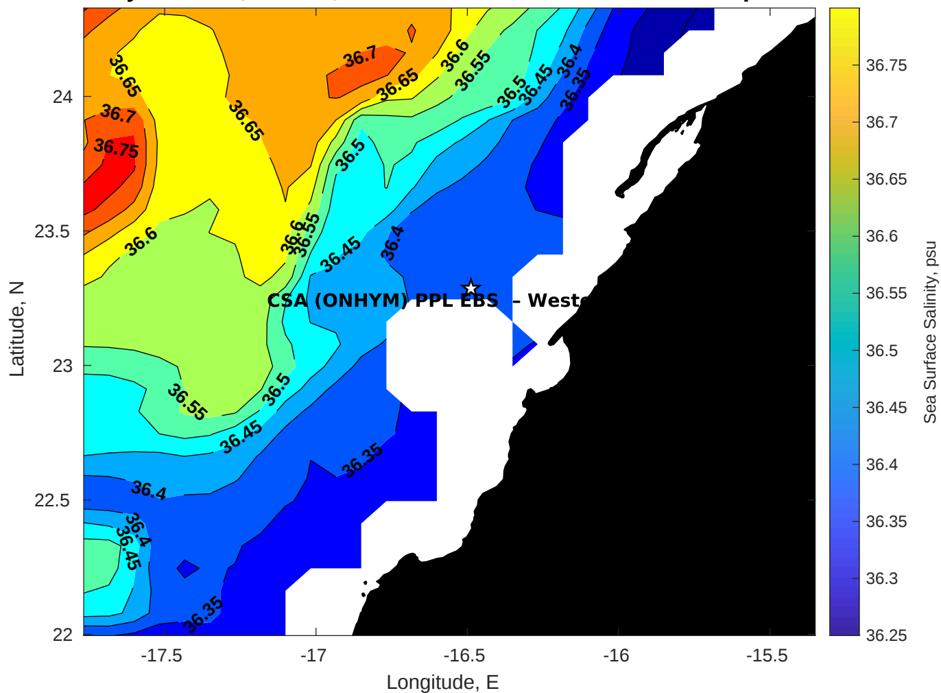
Surface Salinity for CSA (ONHYM) PPL EBS - Western Sahara at 11-Apr-2025 00:00:00
