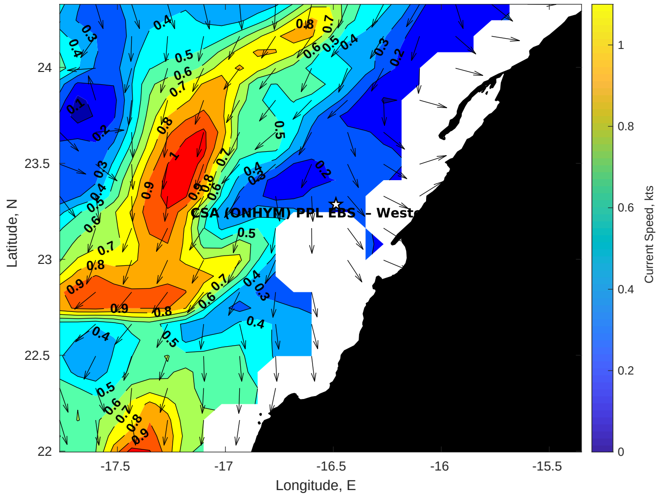
Surface Currents for CSA (ONHYM) PPL EBS - Western Sahara at 11-Apr-2025 00:00:00
