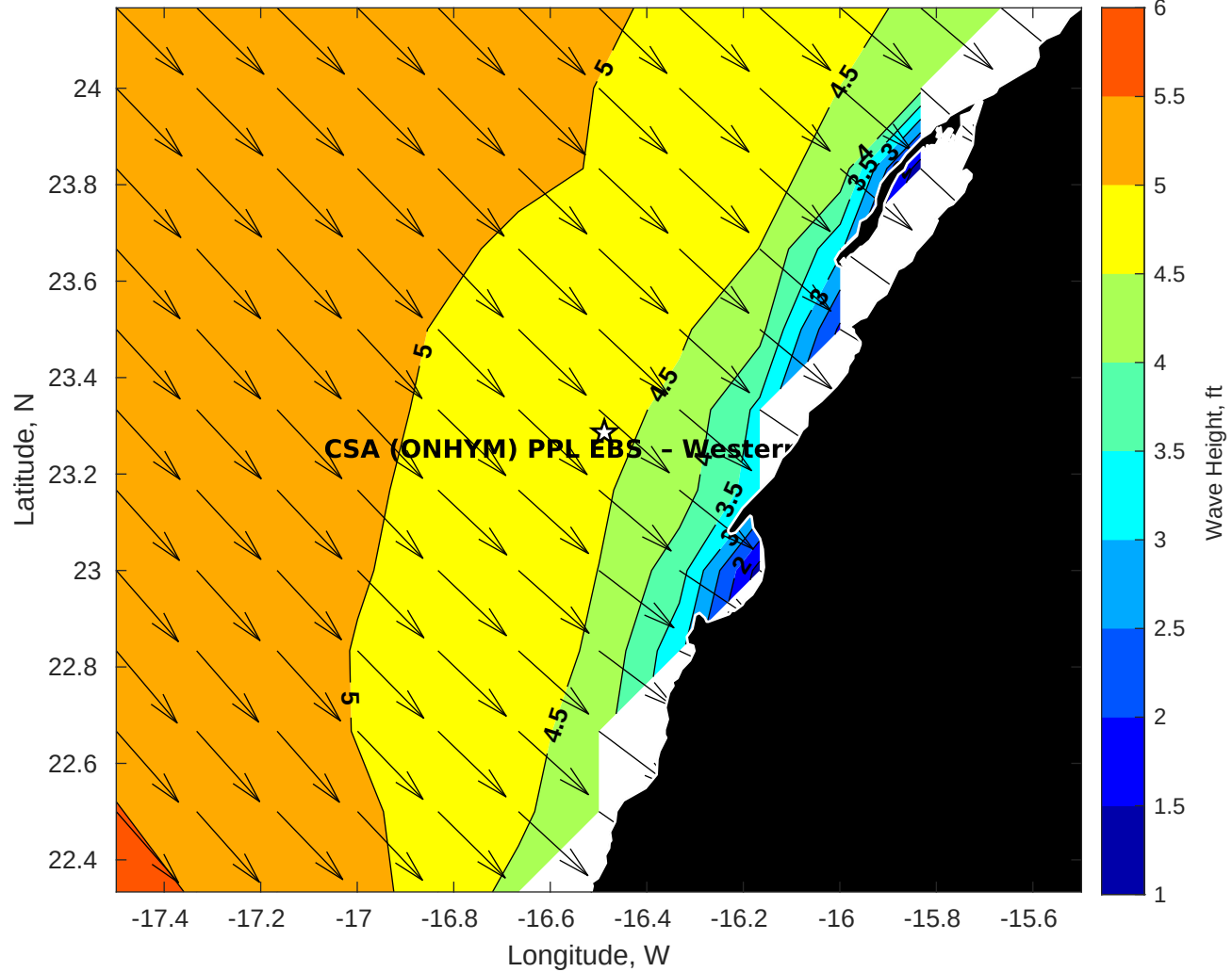
Wave Height (ft) for CSA (ONHYM) PPL EBS - Western Sahara at 12-Apr-2025 09:00:00
