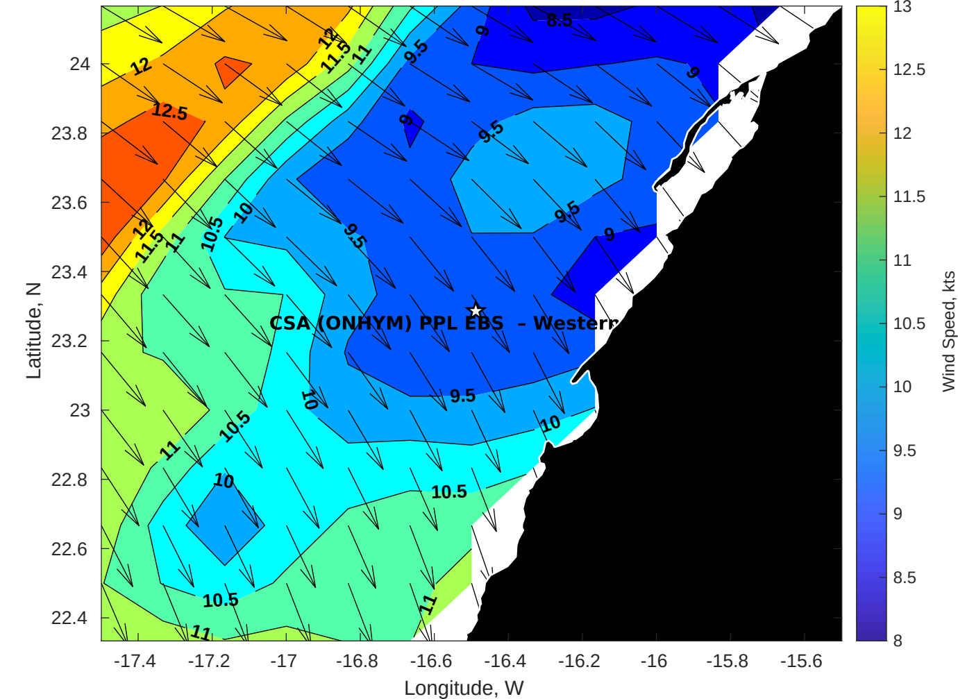
Winds (kts) for CSA (ONHYM) PPL EBS - Western Sahara at 12-Apr-2025 09:00:00
