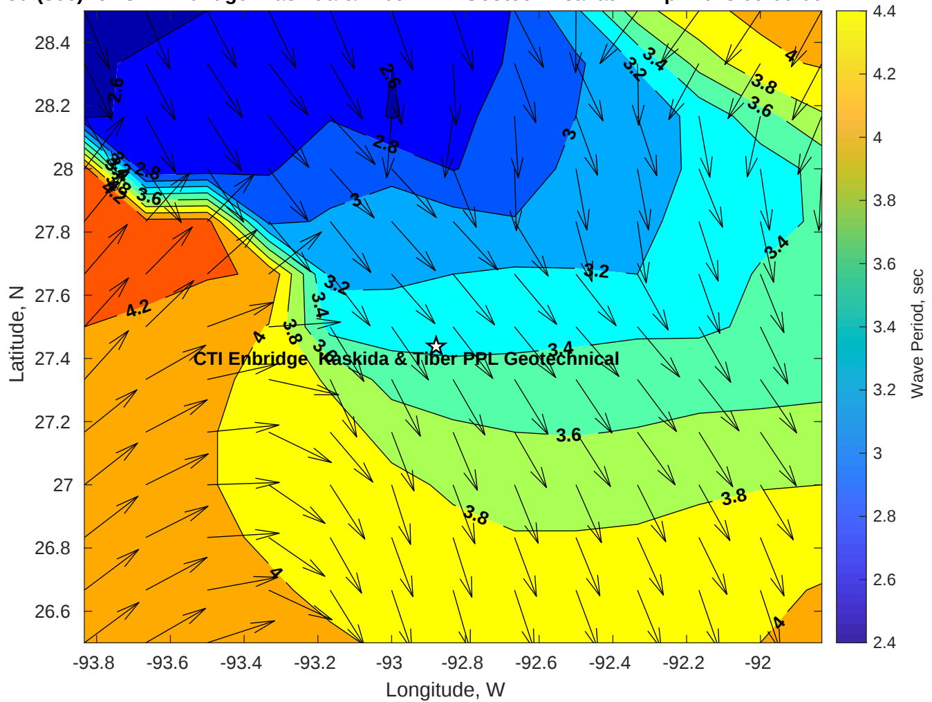
Wave Period (sec) for CTI Enbridge Kaskida & Tiber PPL Geotechnical at 12-Apr-2025 09:00:00
