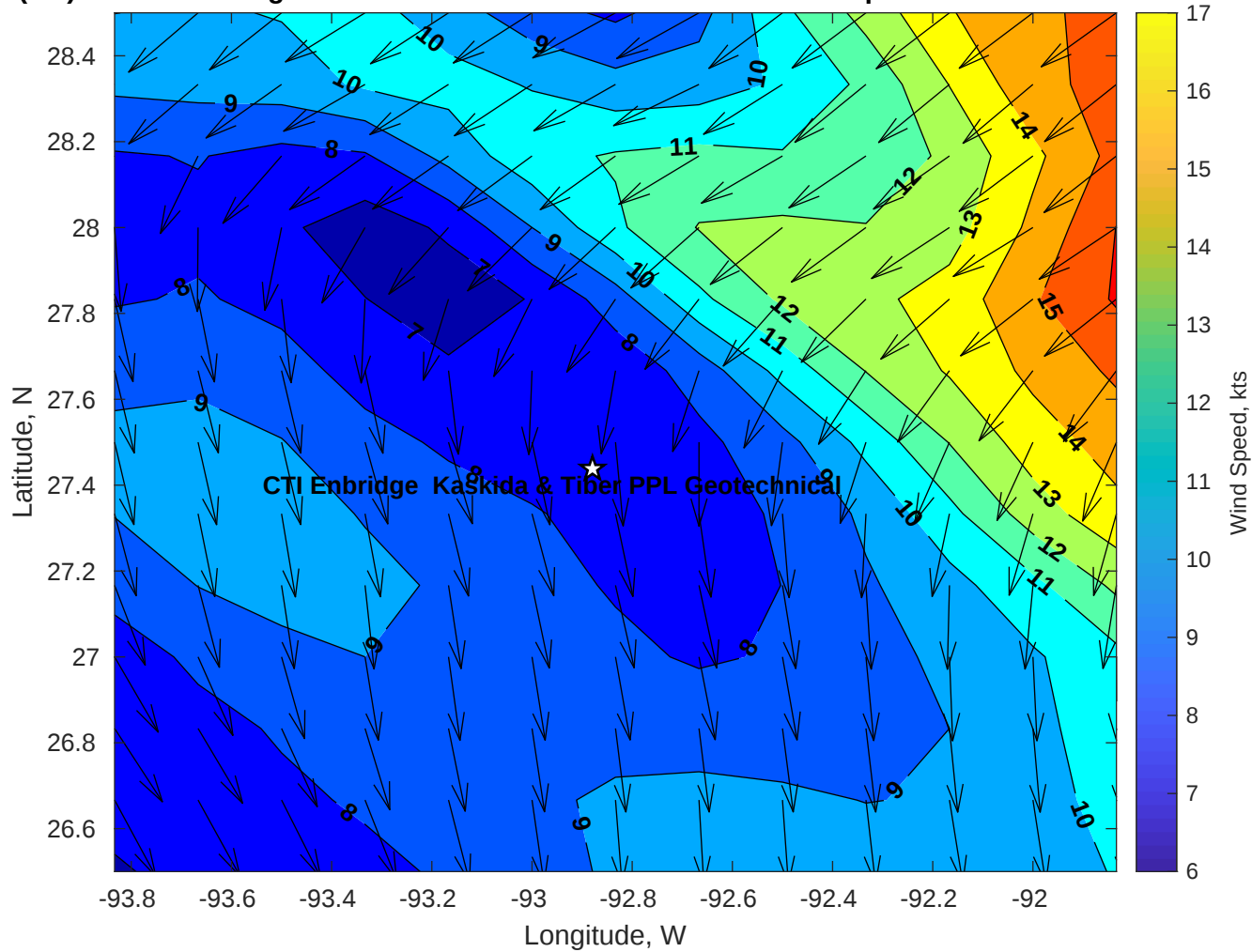
Winds (kts) for CTI Enbridge Kaskida & Tiber PPL Geotechnical at 12-Apr-2025 09:00:00
