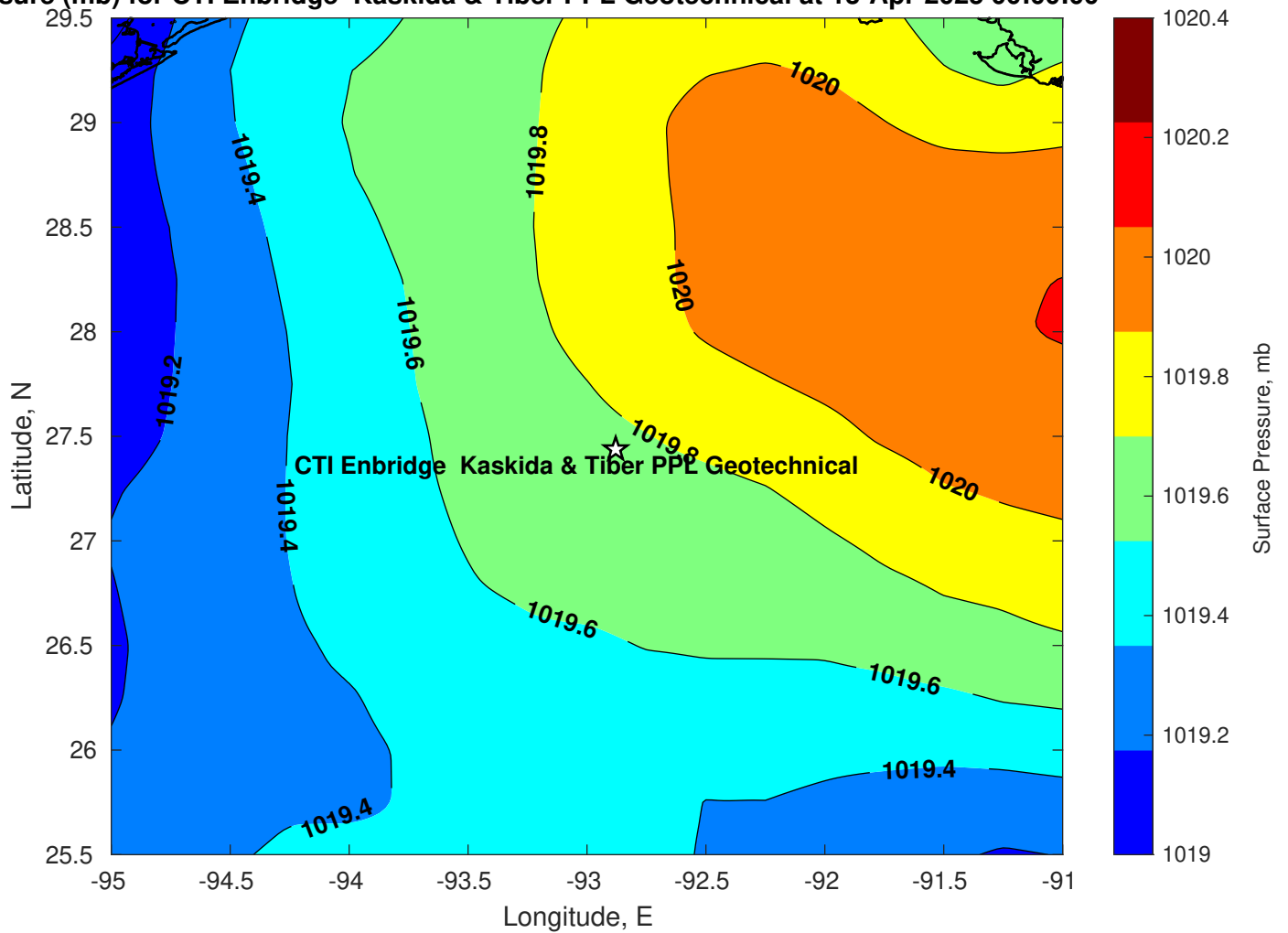
Surface Pressure (mb) for CTI Enbridge Kaskida & Tiber PPL Geotechnical at 13-Apr-2025 00:00:00
