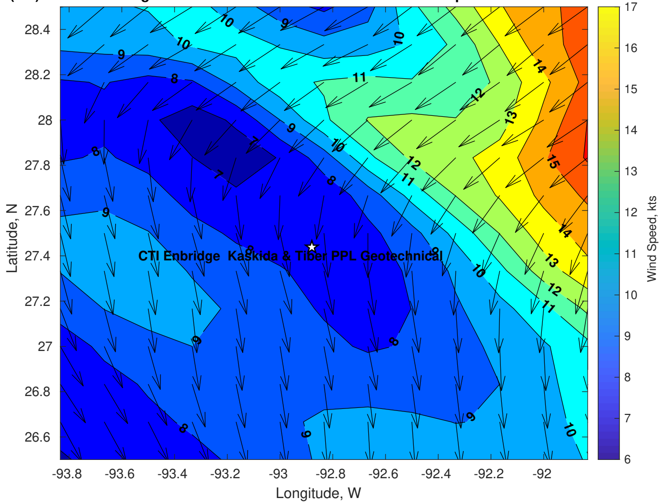
Winds (kts) for CTI Enbridge Kaskida & Tiber PPL Geotechnical at 12-Apr-2025 09:00:00
