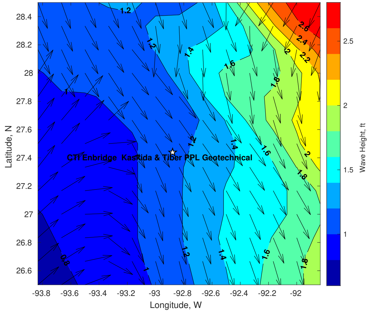
Wave Height (ft) for CTI Enbridge Kaskida & Tiber PPL Geotechnical at 12-Apr-2025 09:00:00
