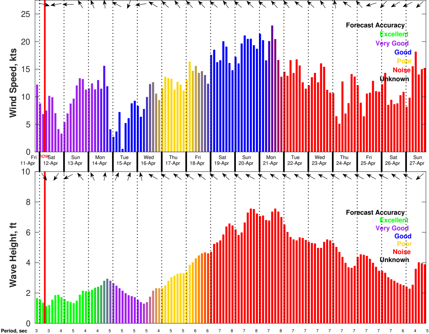
Wind & Wave Forecast for CTI Enbridge Kaskida & Tiber PPL Geotechnical from 11-Apr-2025 20:00:00 to 27-Apr-2025 20:00:00
