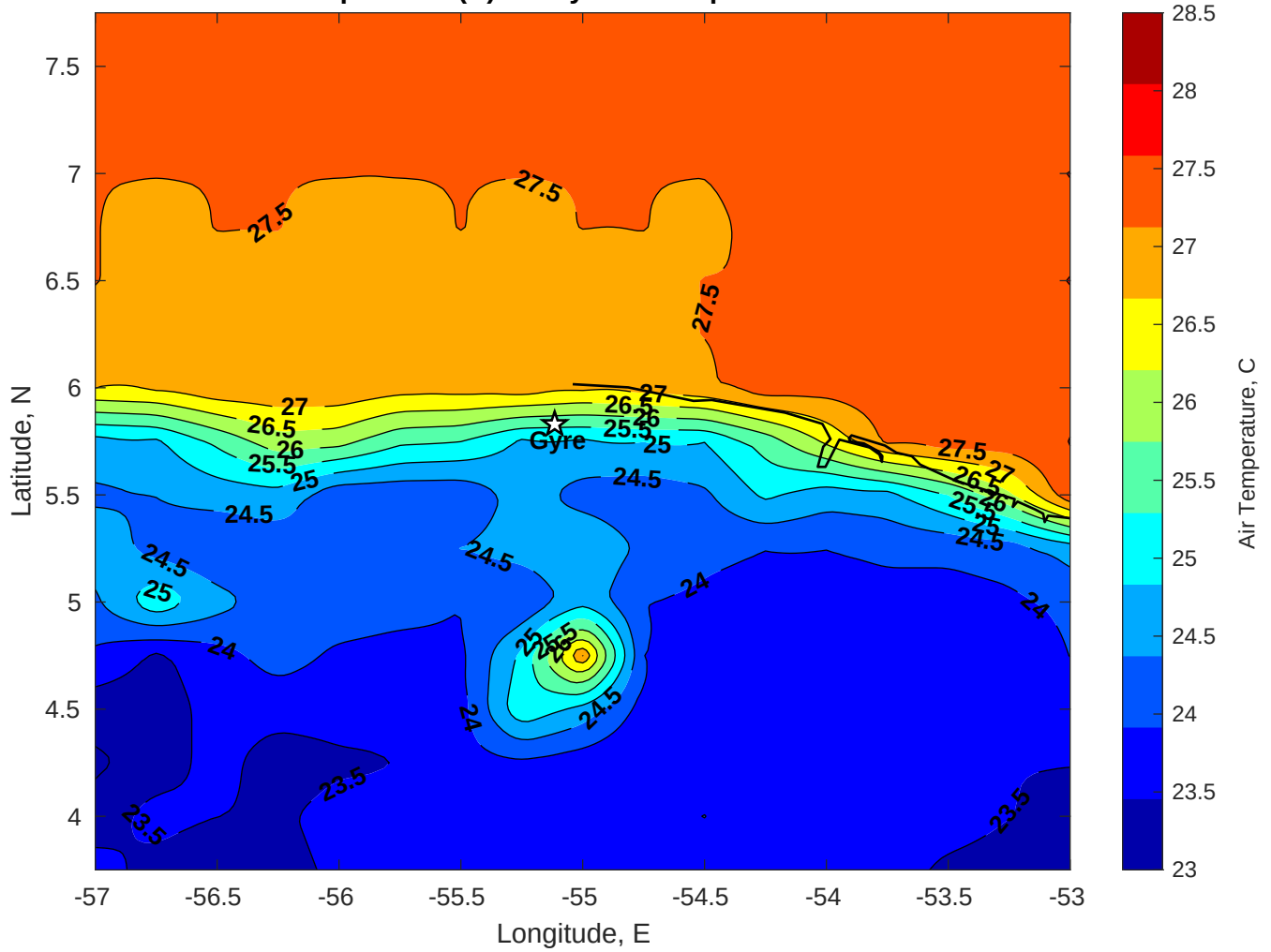
Air Temperature (C) for Gyre at 12-Apr-2025
