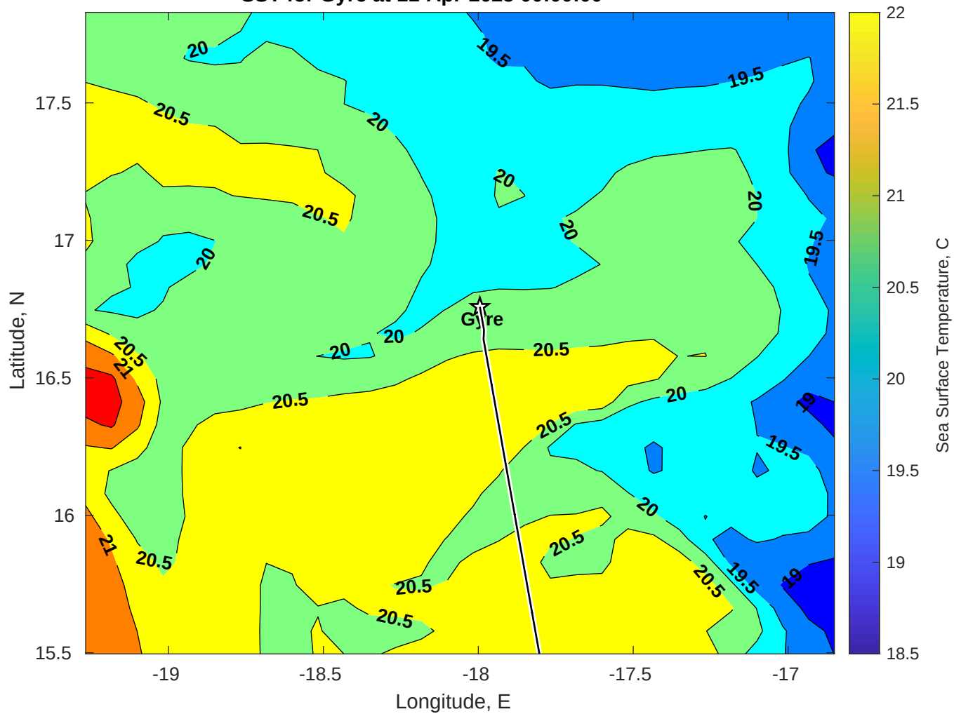
SST for Gyre at 11-Apr-2025 00:00:00
