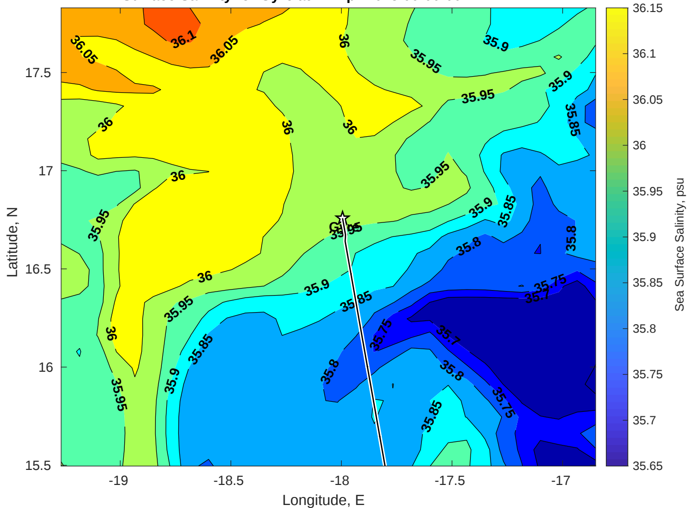
Surface Salinity for Gyre at 11-Apr-2025 00:00:00
