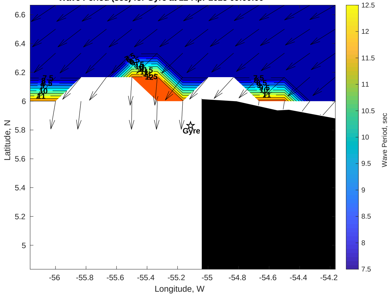
Wave Period (sec) for Gyre at 12-Apr-2025 09:00:00
