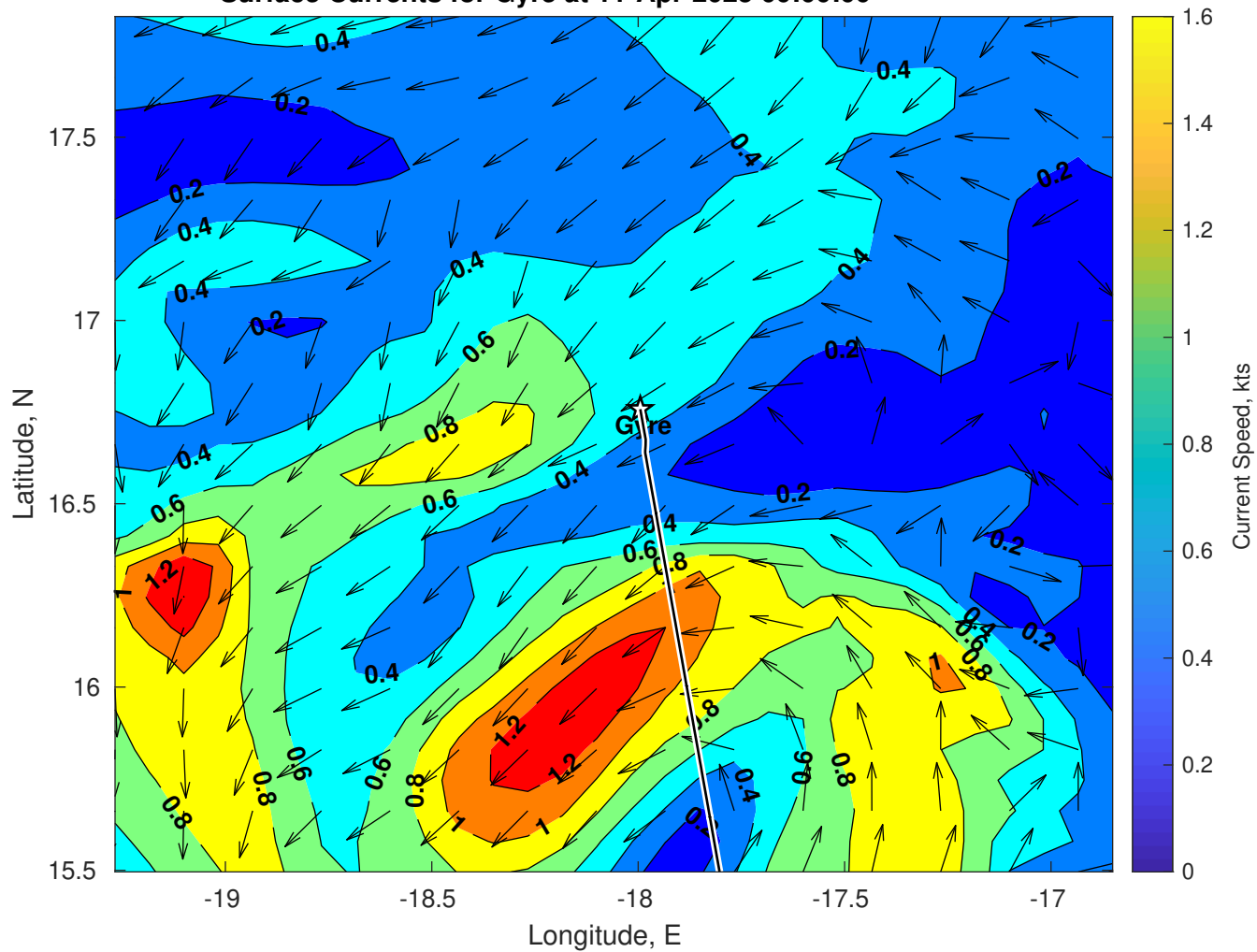
Surface Currents for Gyre at 11-Apr-2025 00:00:00
