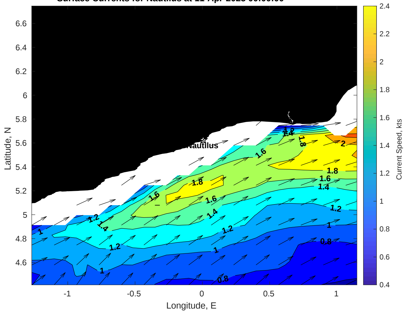
Surface Currents for Nautilus at 11-Apr-2025 00:00:00
