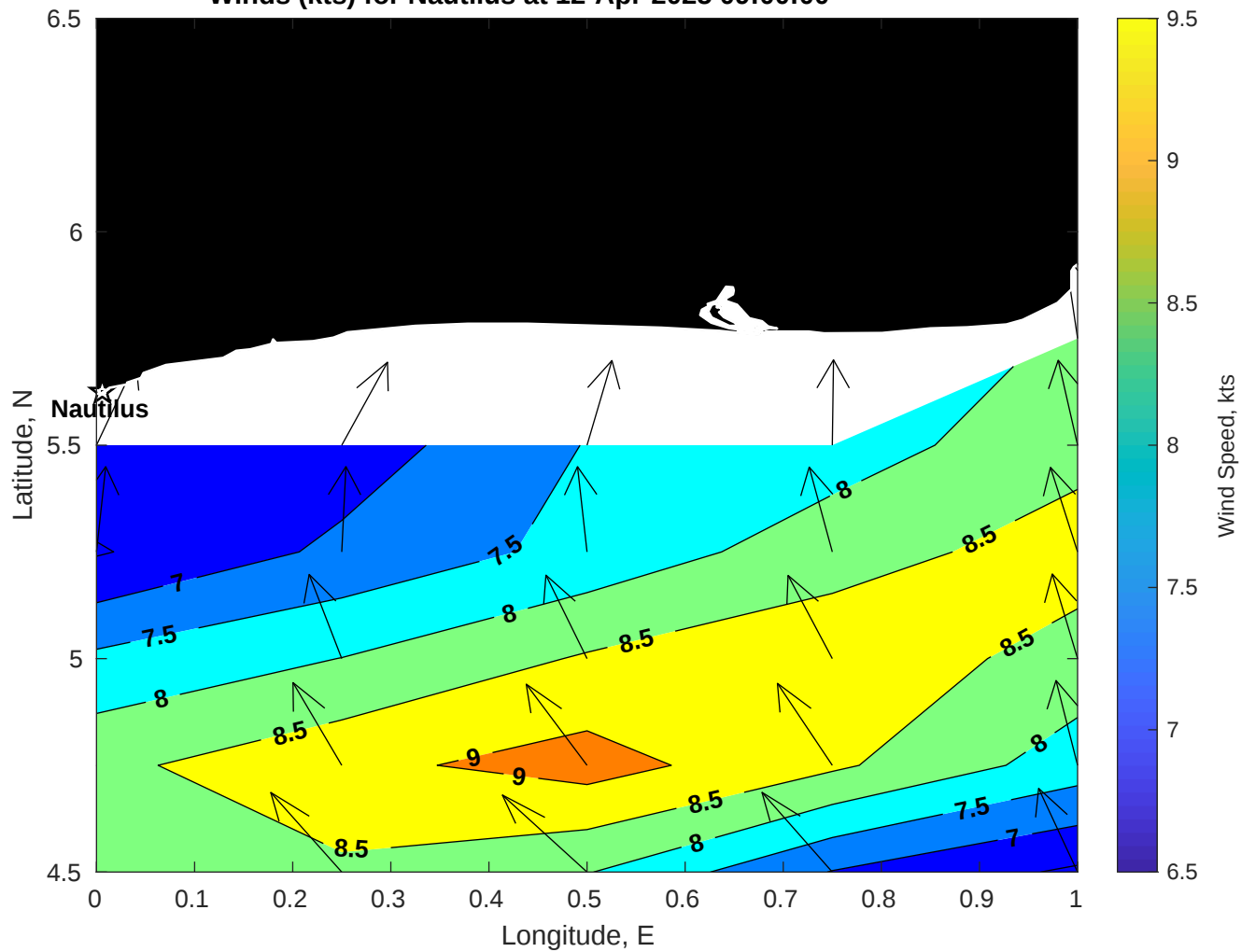
Winds (kts) for Nautilus at 12-Apr-2025 09:00:00
