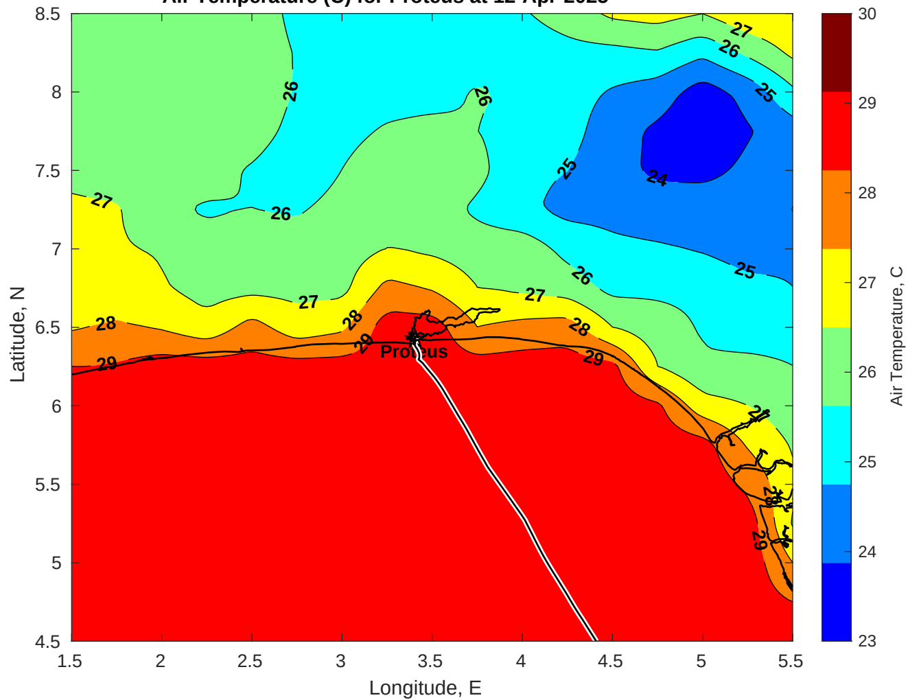
Air Temperature (C) for Proteus at 12-Apr-2025
