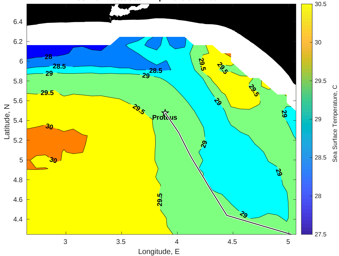
SST for Proteus at 11-Apr-2025 00:00:00
