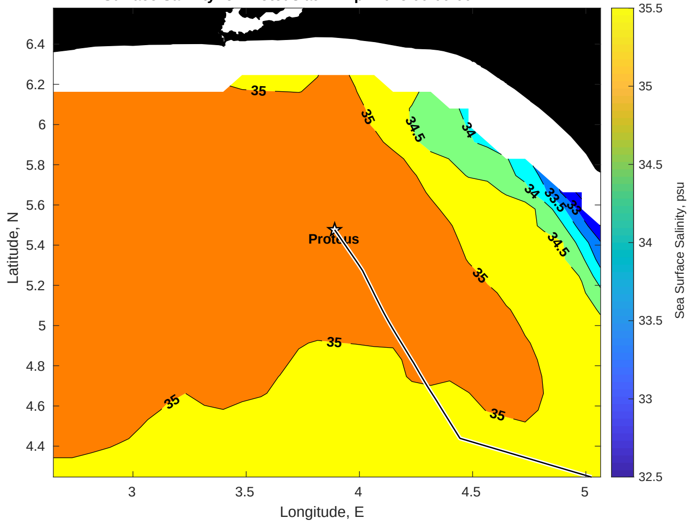
Surface Salinity for Proteus at 11-Apr-2025 00:00:00
