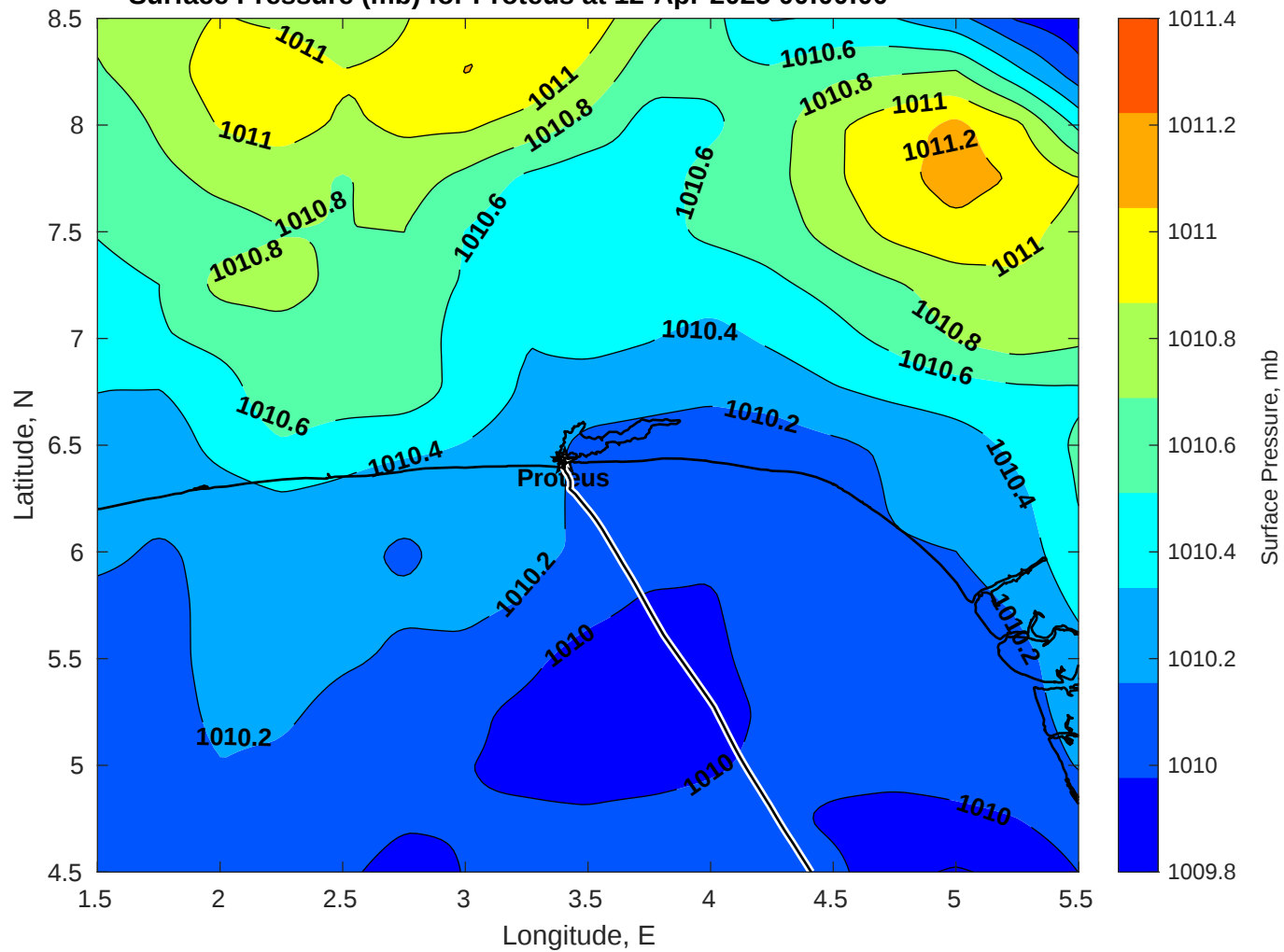
Surface Pressure (mb) for Proteus at 12-Apr-2025 00:00:00
