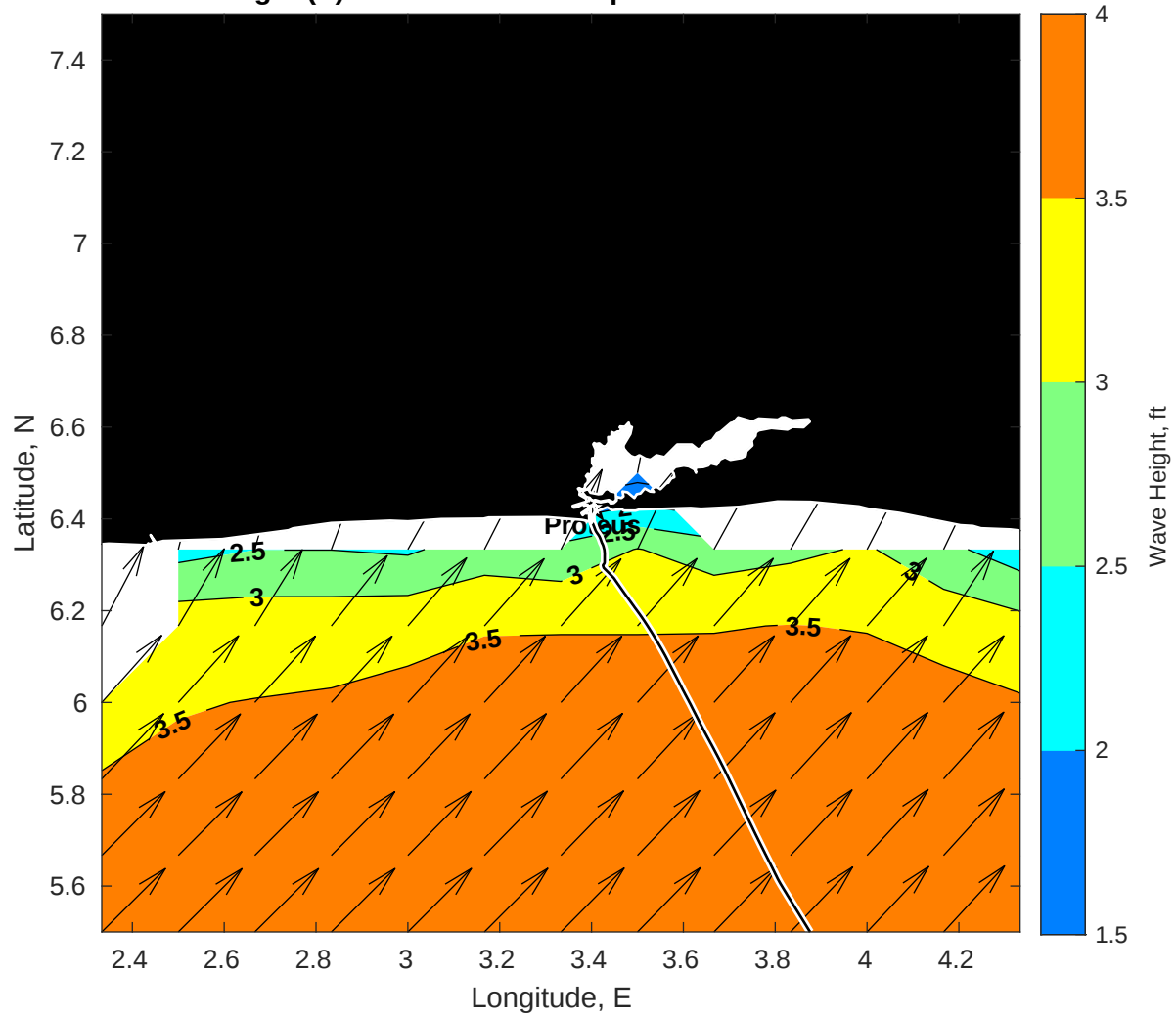
Wave Height (ft) for Proteus at 12-Apr-2025 09:00:00
