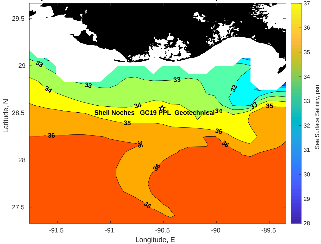
Surface Salinity for Shell Noches GC19 PPL Geotechnical at 11-Apr-2025 00:00:00
