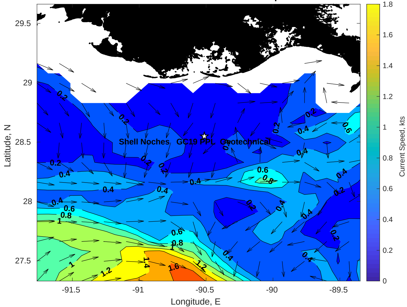
Surface Currents for Shell Noches GC19 PPL Geotechnical at 11-Apr-2025 00:00:00
