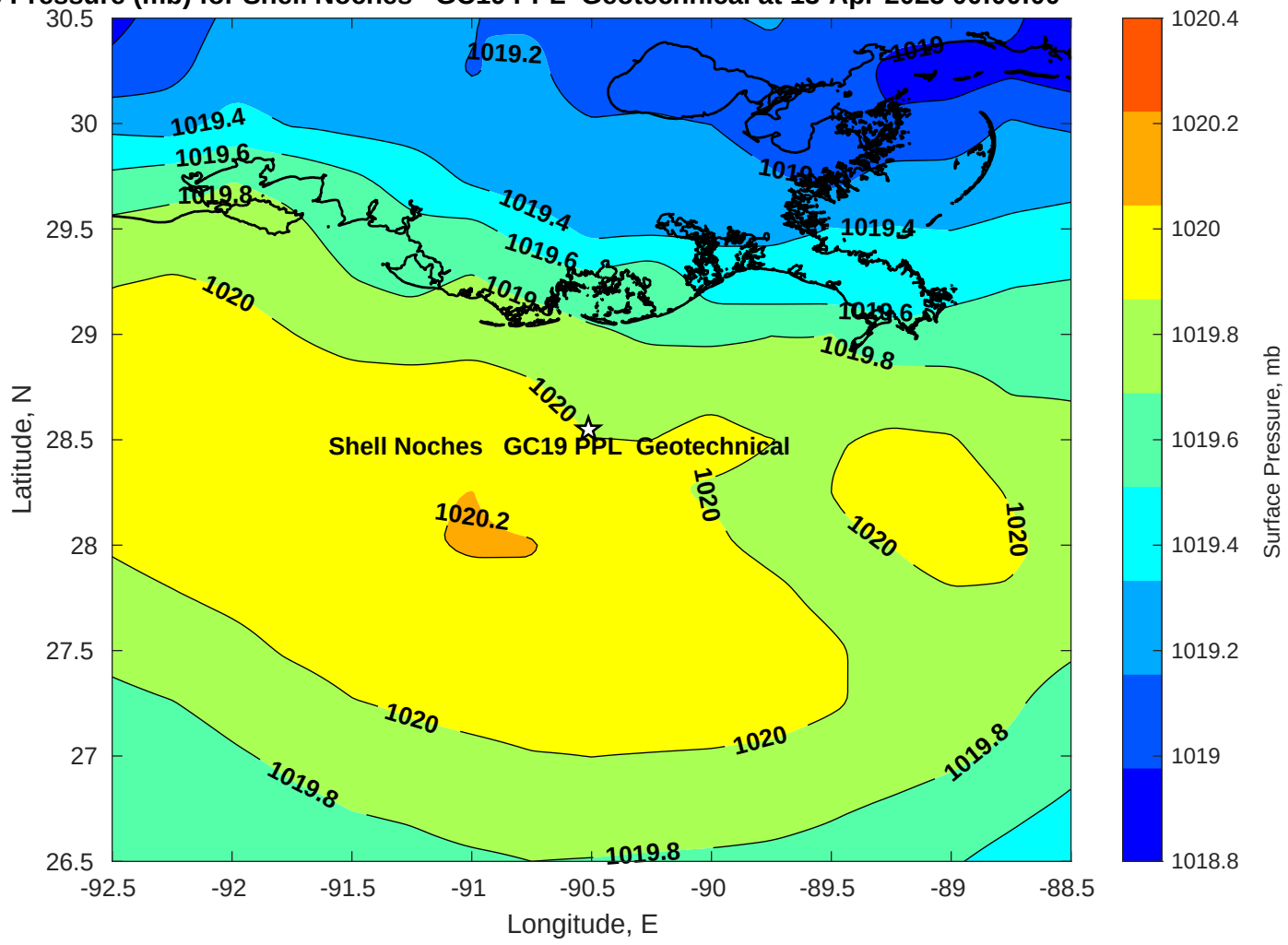
Surface Pressure (mb) for Shell Noches GC19 PPL Geotechnical at 13-Apr-2025 00:00:00
