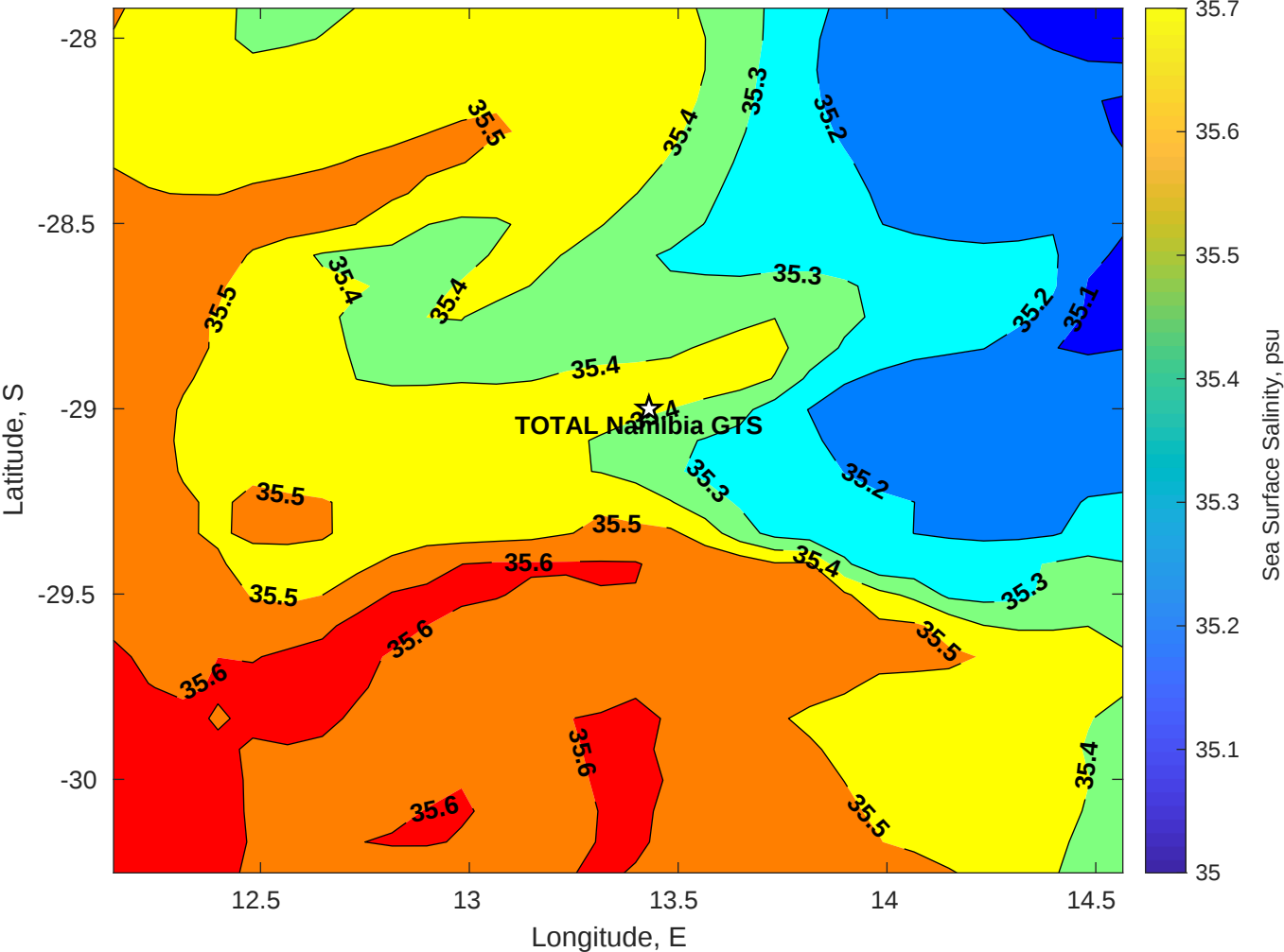
Surface Salinity for TOTAL Namibia GTS at 11-Apr-2025 00:00:00
