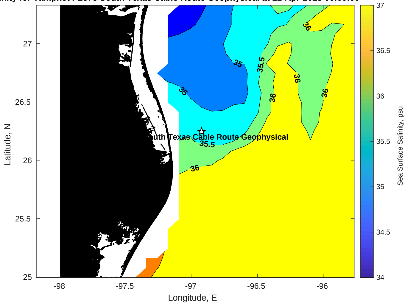
Surface Salinity for Tampnet P2378 South Texas Cable Route Geophysical at 11-Apr-2025 00:00:00
