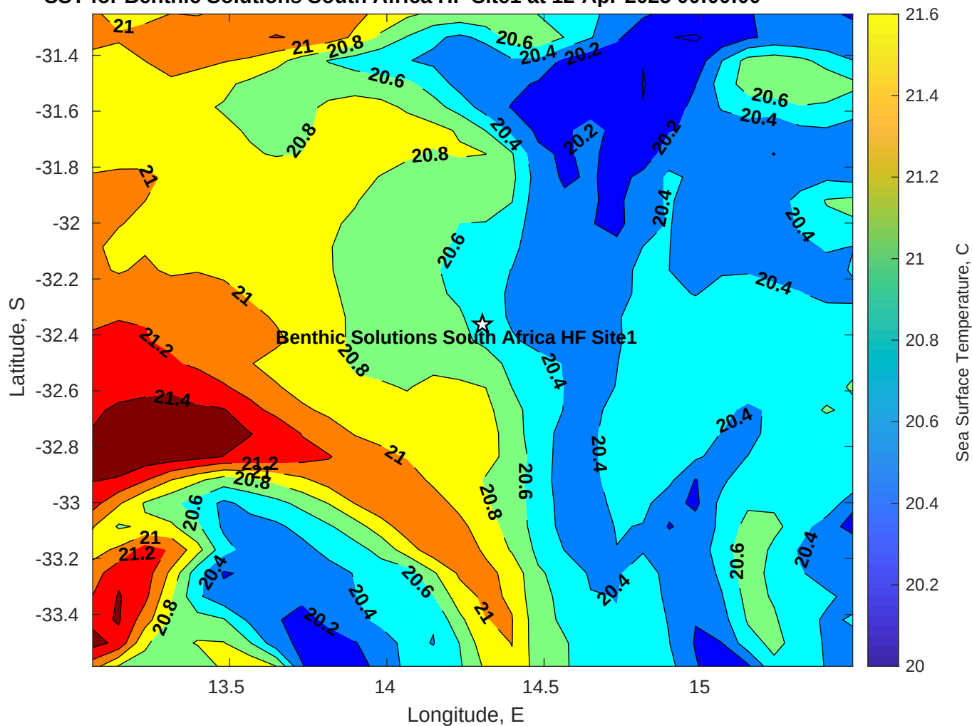
SST for Benthic Solutions South Africa HF Site1 at 12-Apr-2025 00:00:00
