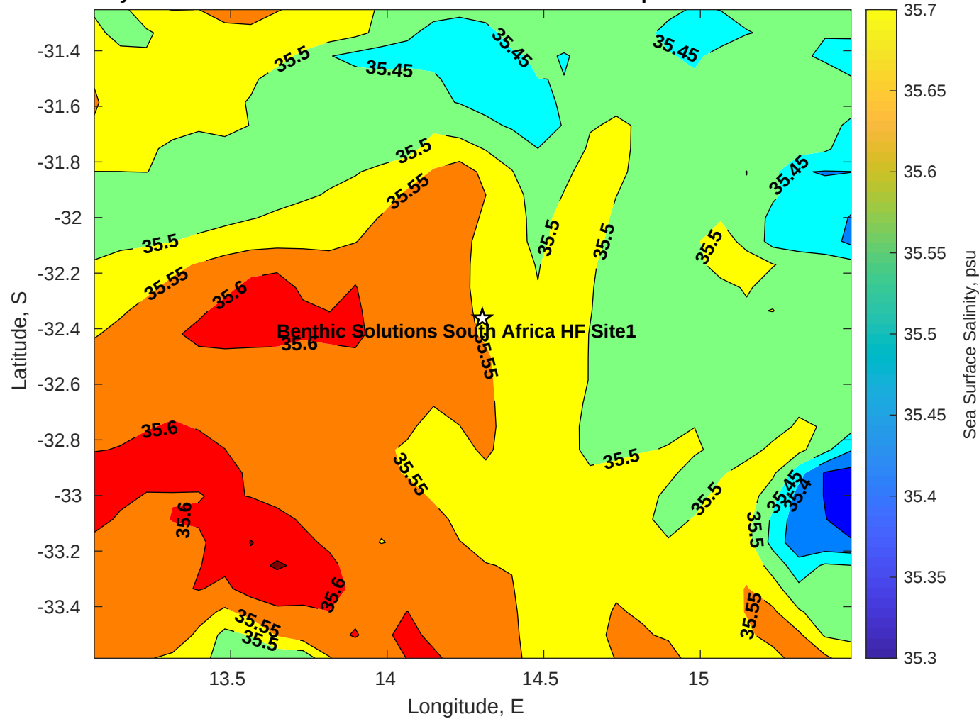
Surface Salinity for Benthic Solutions South Africa HF Site1 at 12-Apr-2025 00:00:00
