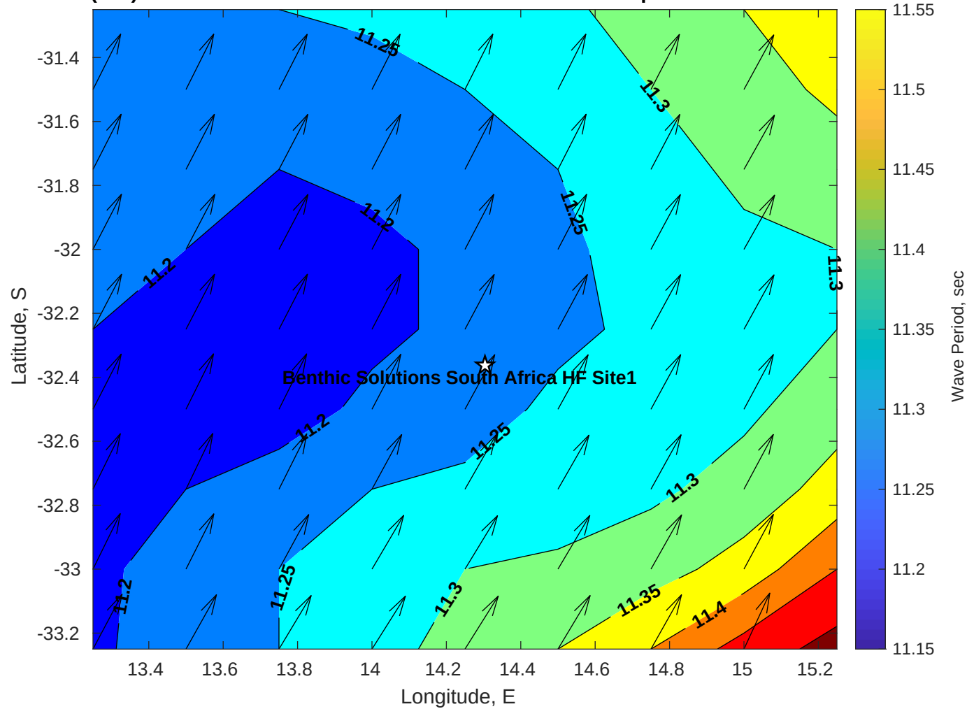
Wave Period (sec) for Benthic Solutions South Africa HF Site1 at 13-Apr-2025 09:00:00
