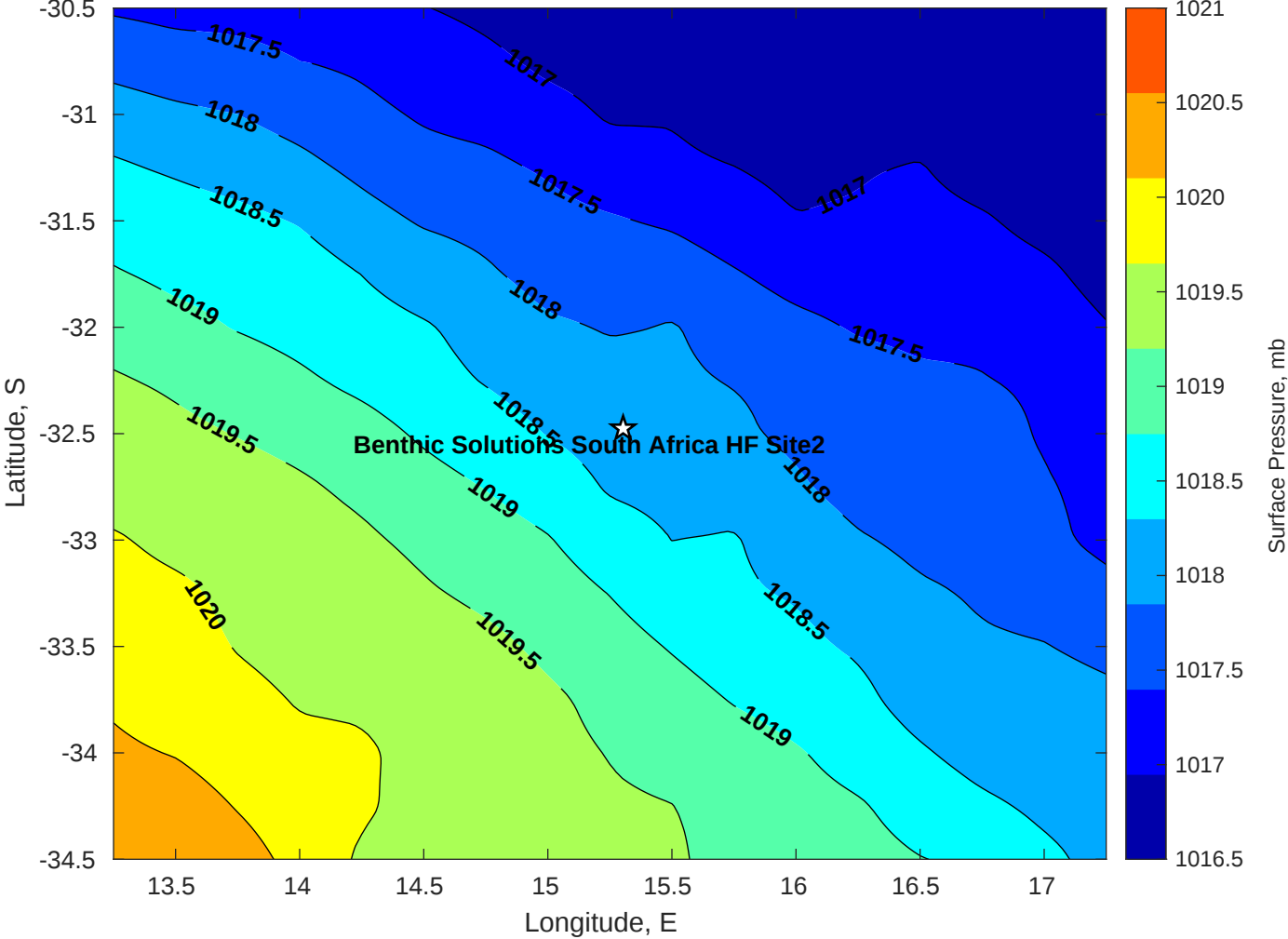
Surface Pressure (mb) for Benthic Solutions South Africa HF Site2 at 13-Apr-2025 00:00:00
