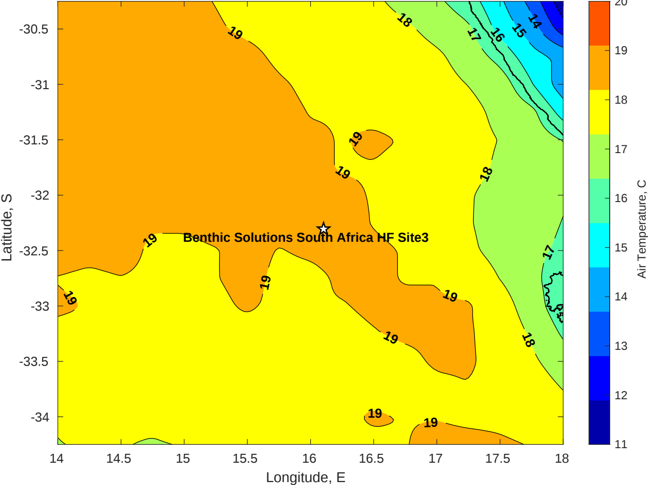
Air Temperature (C) for Benthic Solutions South Africa HF Site3 at 13-Apr-2025
