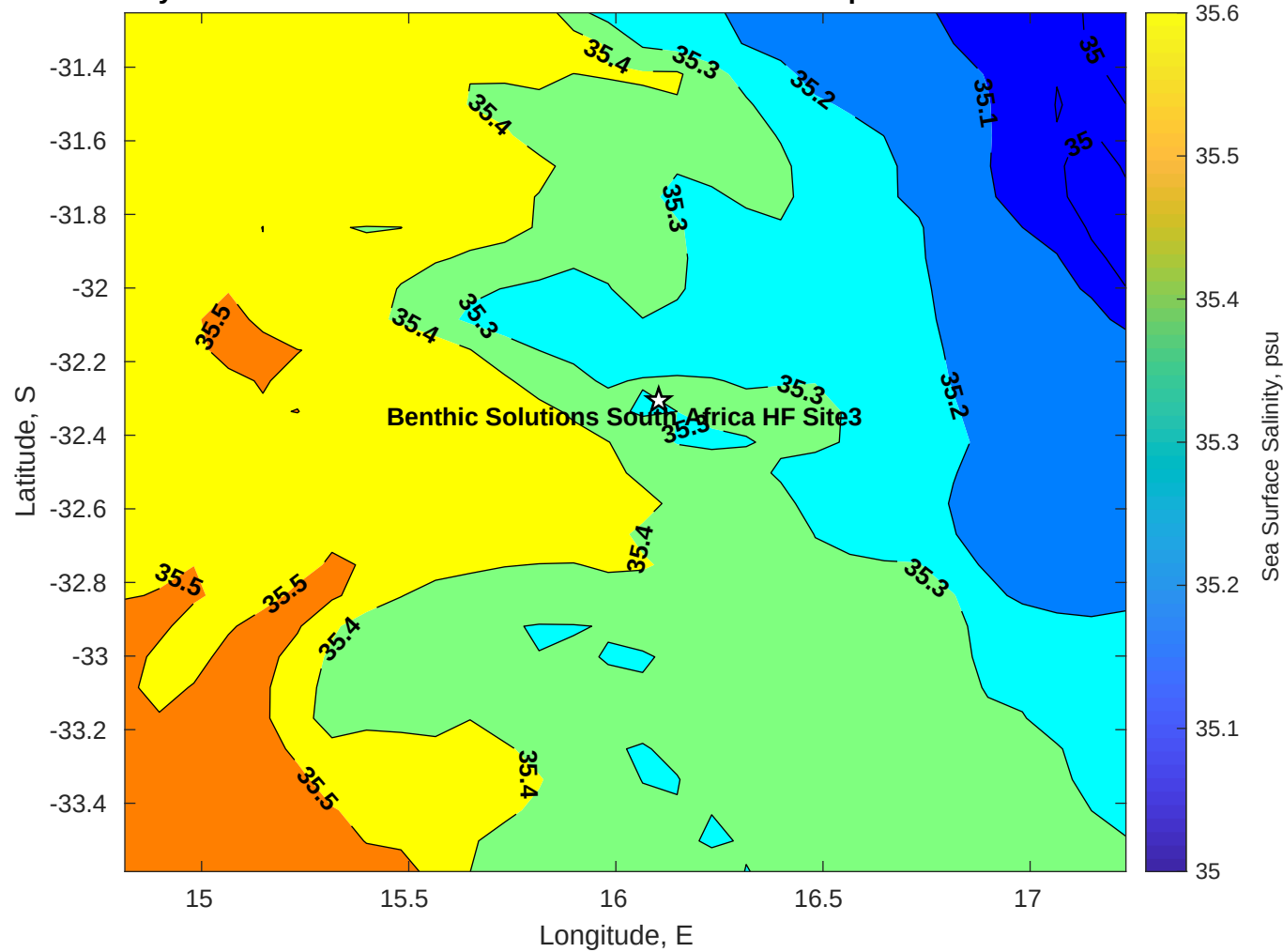
Surface Salinity for Benthic Solutions South Africa HF Site3 at 12-Apr-2025 00:00:00
