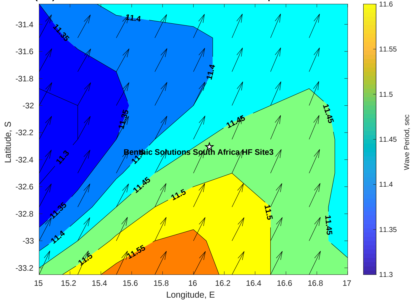
Wave Period (sec) for Benthic Solutions South Africa HF Site3 at 13-Apr-2025 09:00:00
