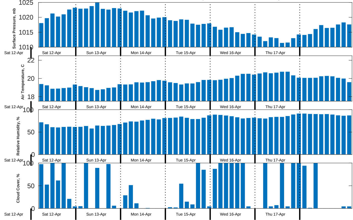
Met Forecast for Benthic Solutions South Africa HF Site3 from 13-Apr-2025 00:00:00 to 20-Apr-2025 00:00:00
